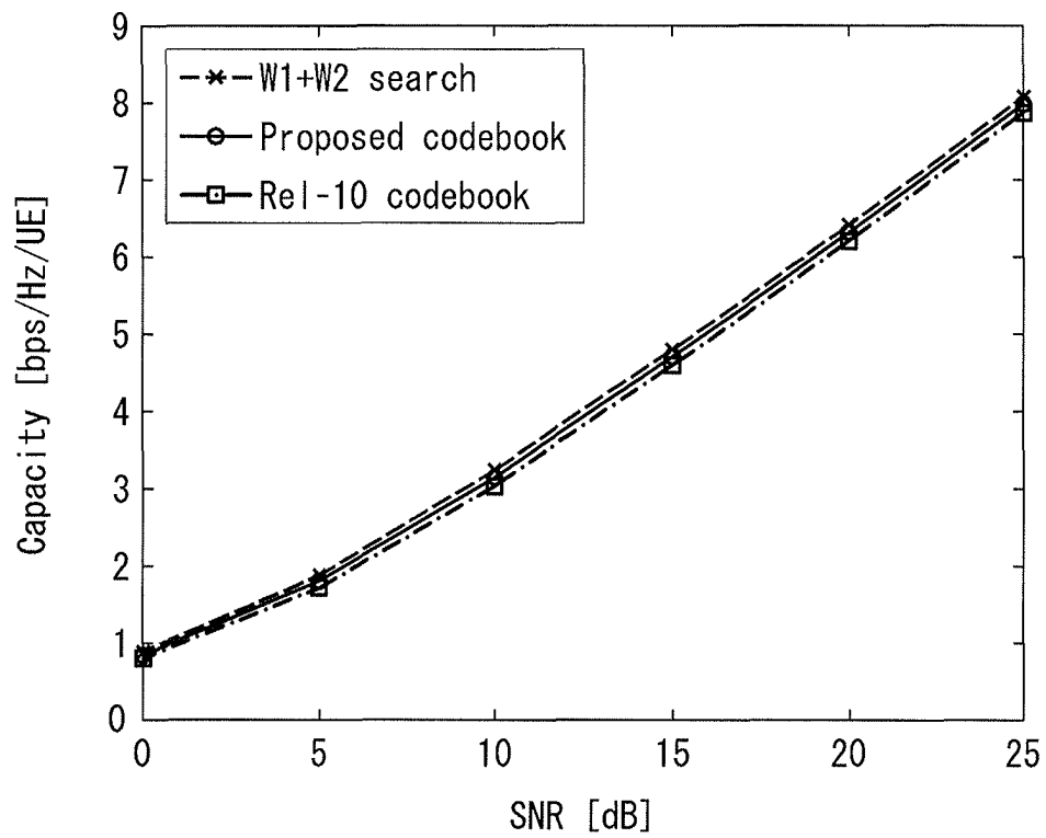
(a) Channel capacity upon single rank transmission
