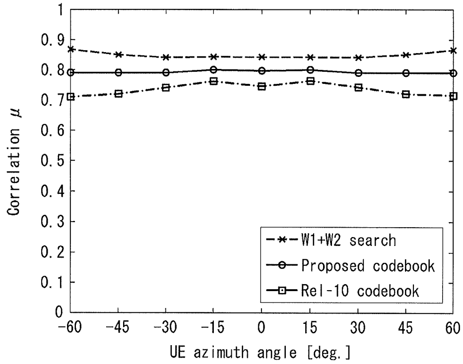
(a) Correlation upon single rank transmission \mu
