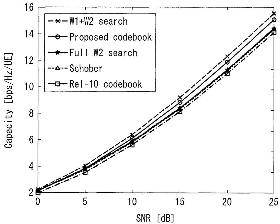
(b) Channel capacity upon dual rank transmission
