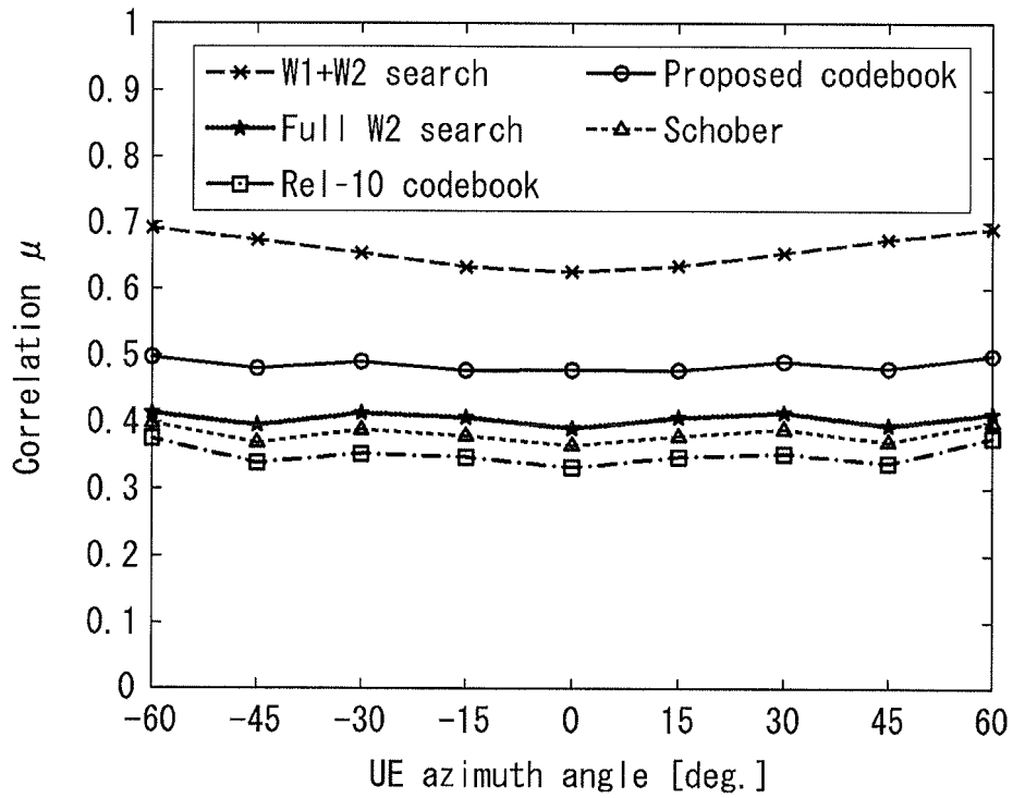
(b) Correlation upon dual rank transmission \mu
