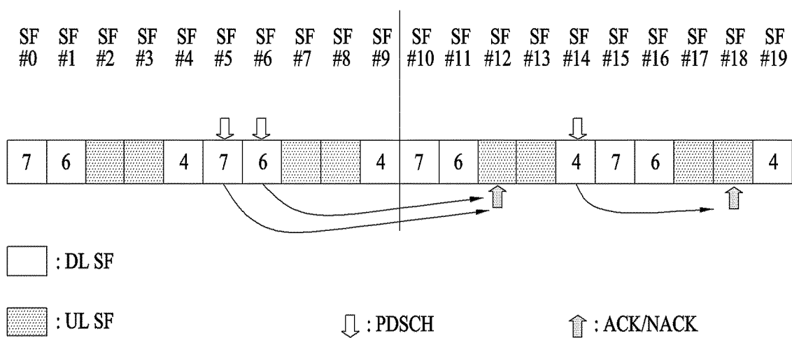
PDSCH-ACK/NACK timing (UL-DL configuration #1)
