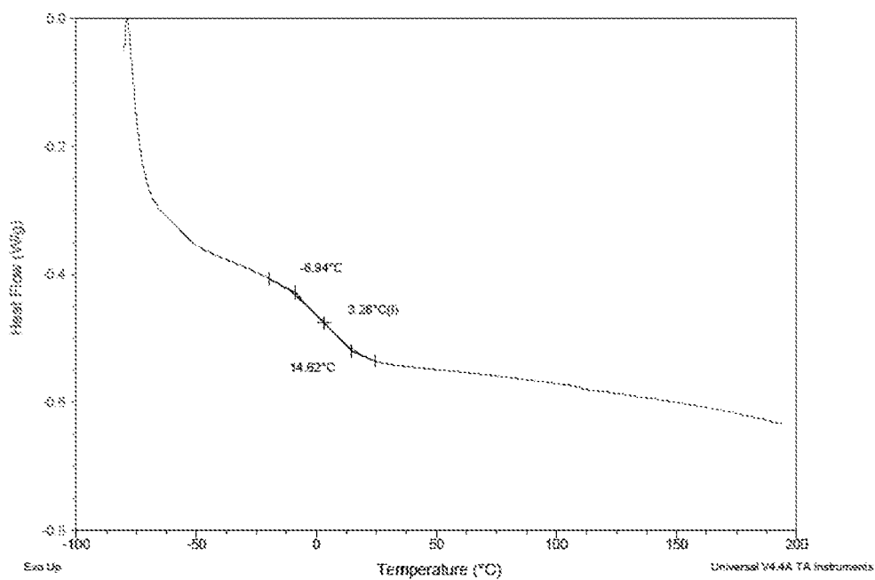
Figure 21a. DSC graph of reference foam (Formulation #1 in Tables 2B-5B)
