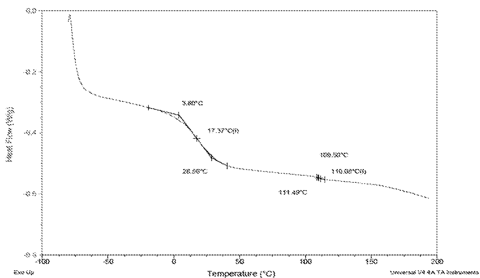
Figure 23b. DSC graph of foam prepared with a mixture of three different Novomer Polyols (Formulation #6 in Table 5B)
