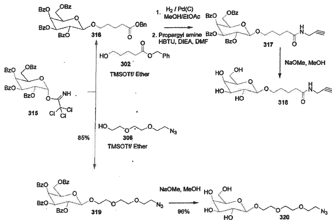
Scheme 13
