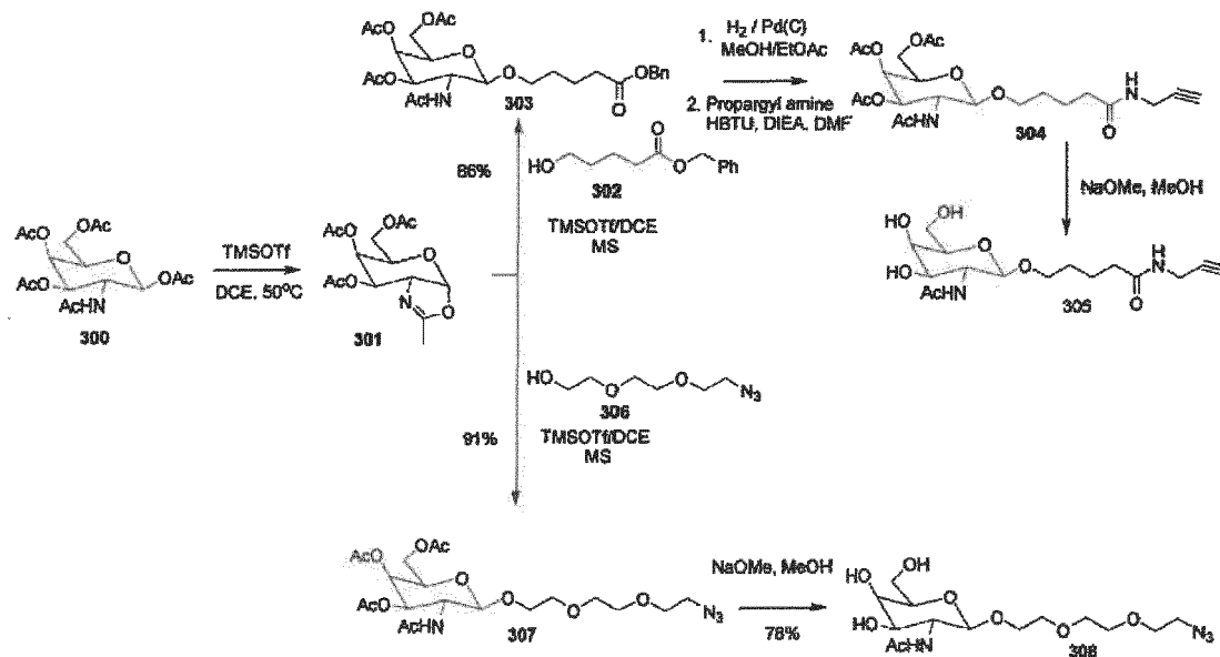
Scheme 10
