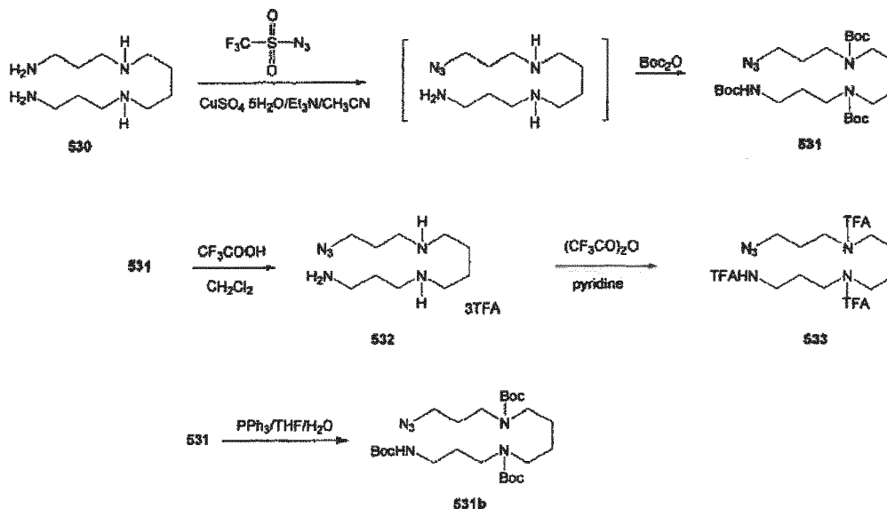
Scheme 35
