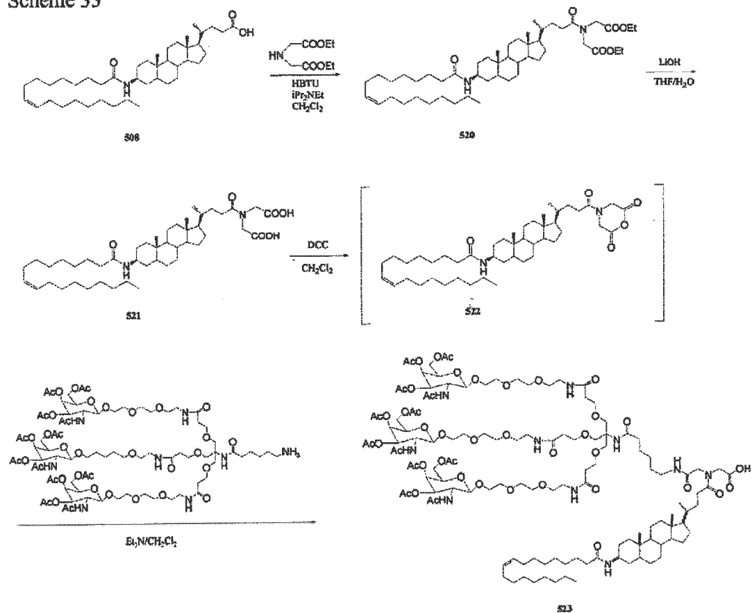
Scheme 33
