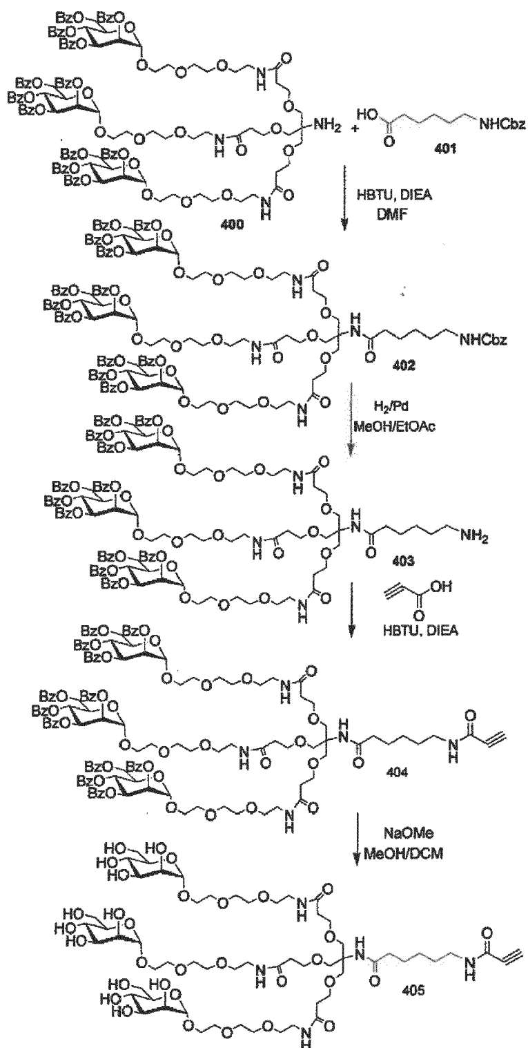
Scheme 16
