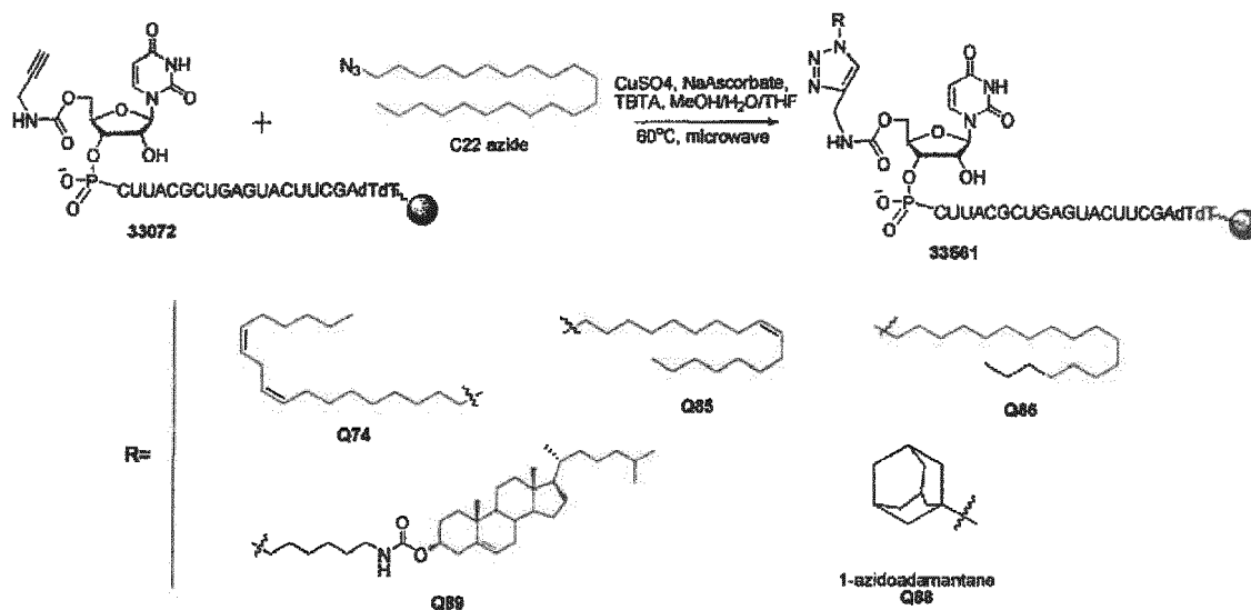
Scheme 39
