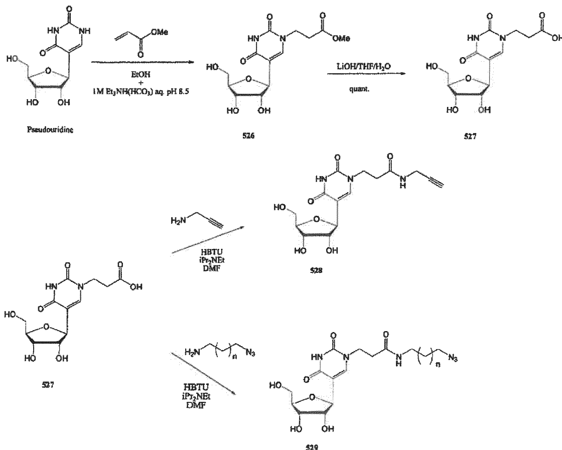
Scheme 34
