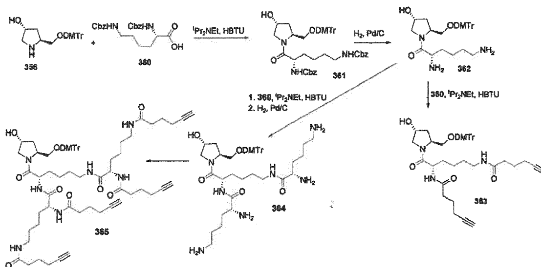
Scheme 26
