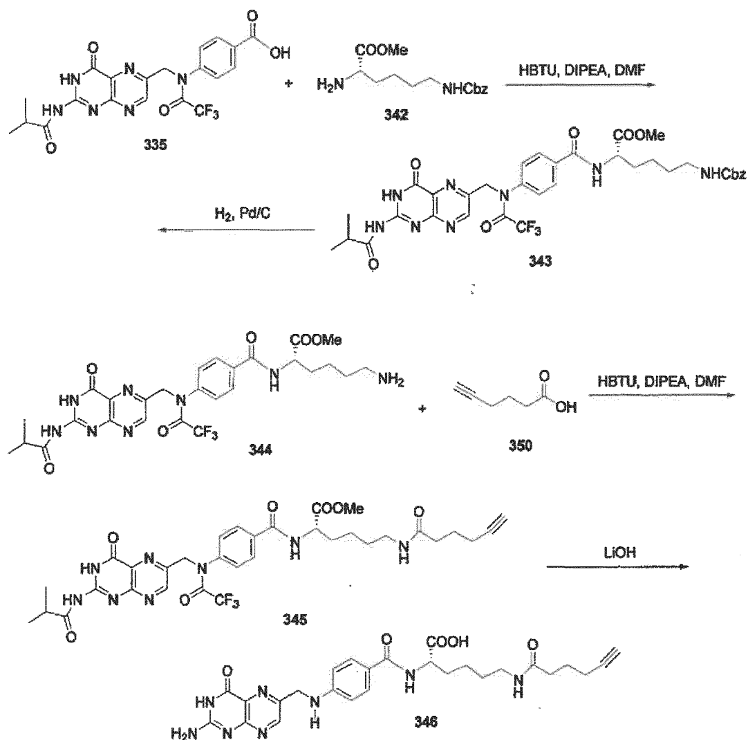
Scheme 22
