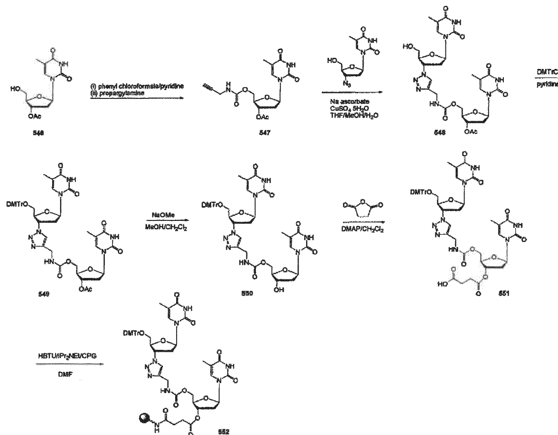
Scheme 42
