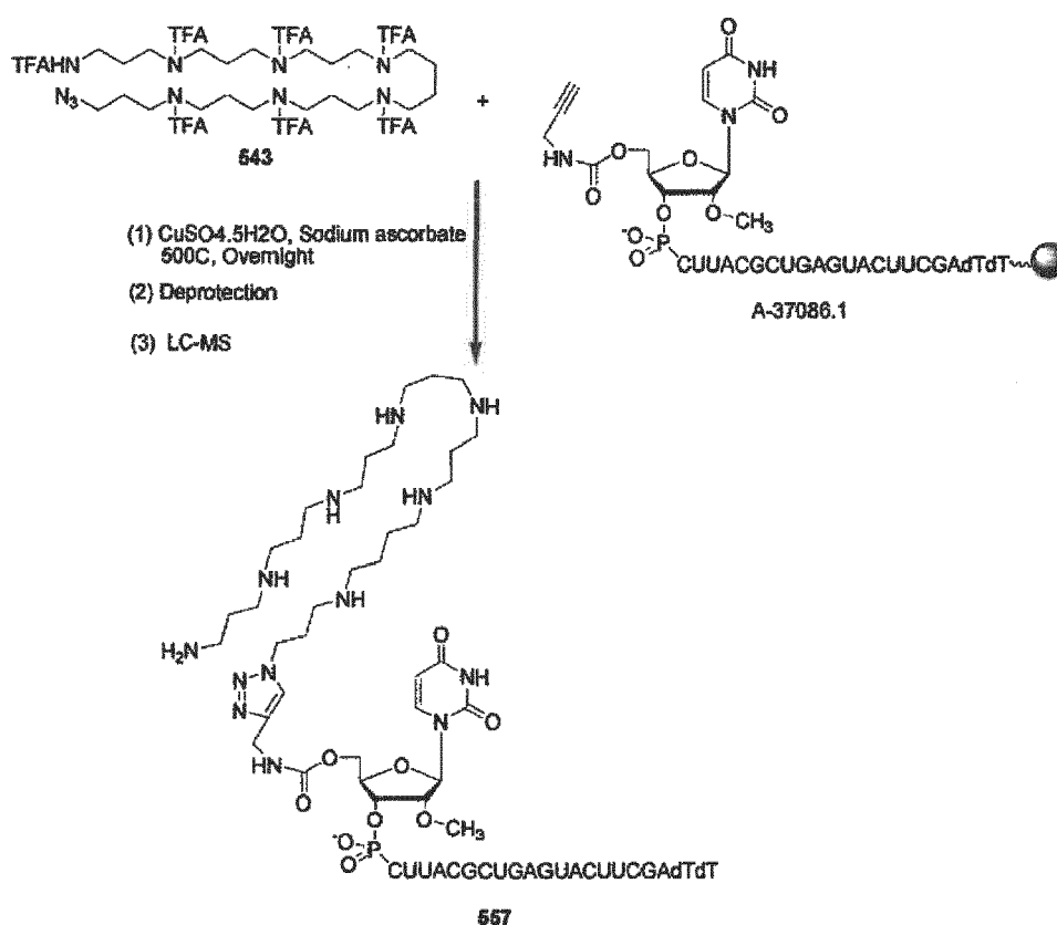
Scheme 46
