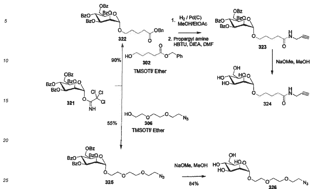
Scheme 14
