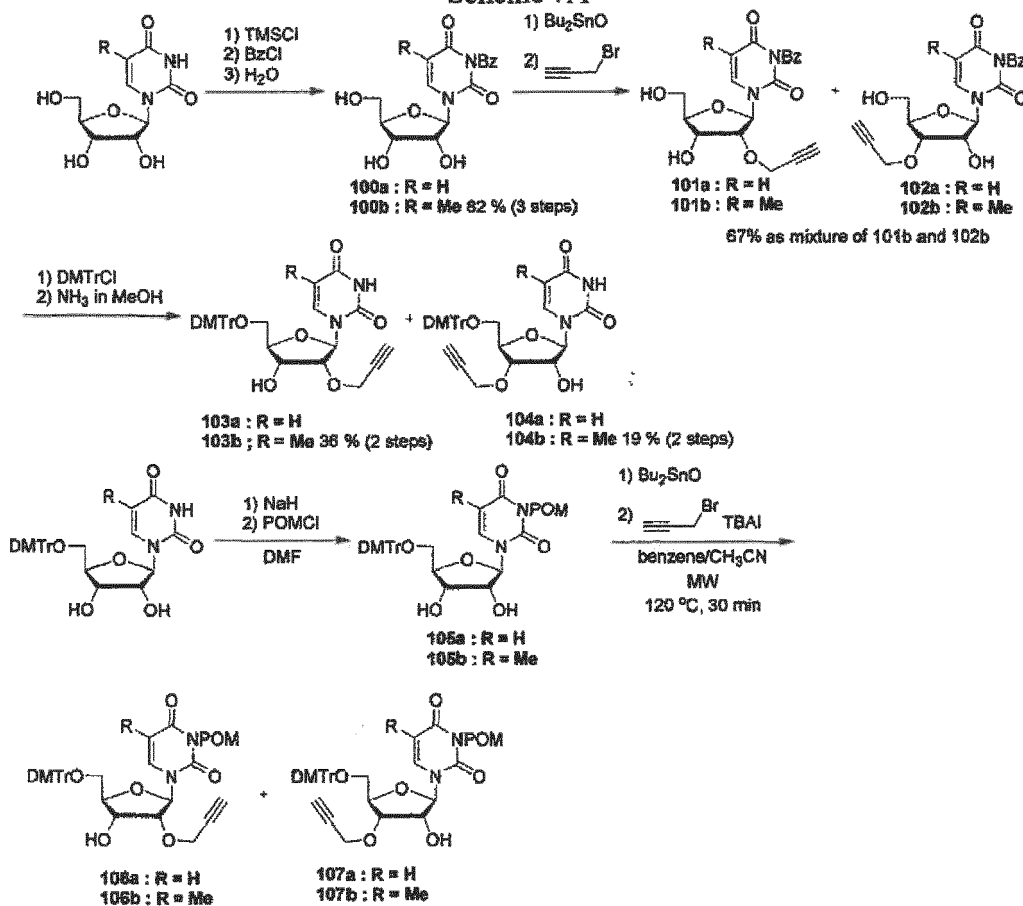
Scheme 7A
