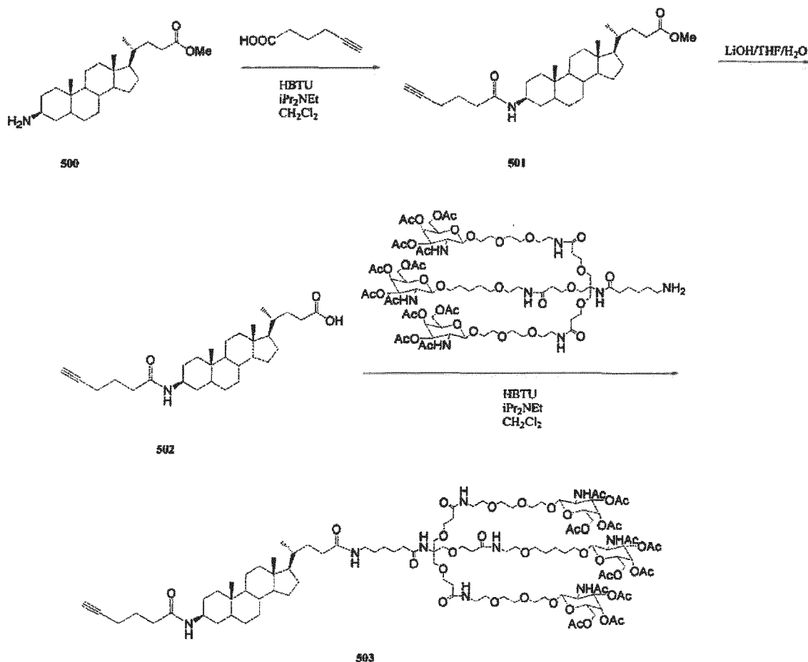
Scheme 28
