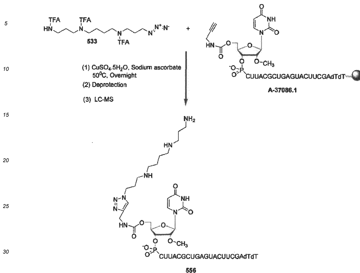
Scheme 45
