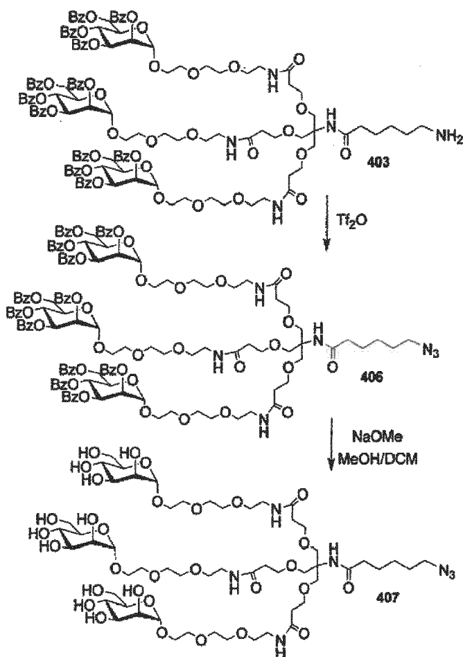
Scheme 17
