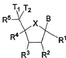
Formula (Ia)
