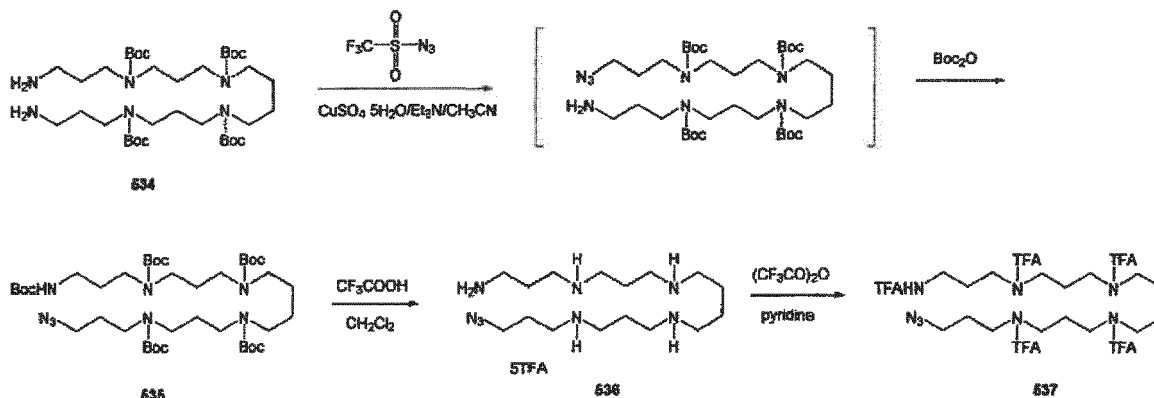
Scheme 36
