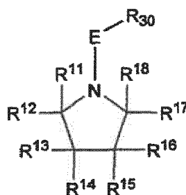
Formula (VI)
