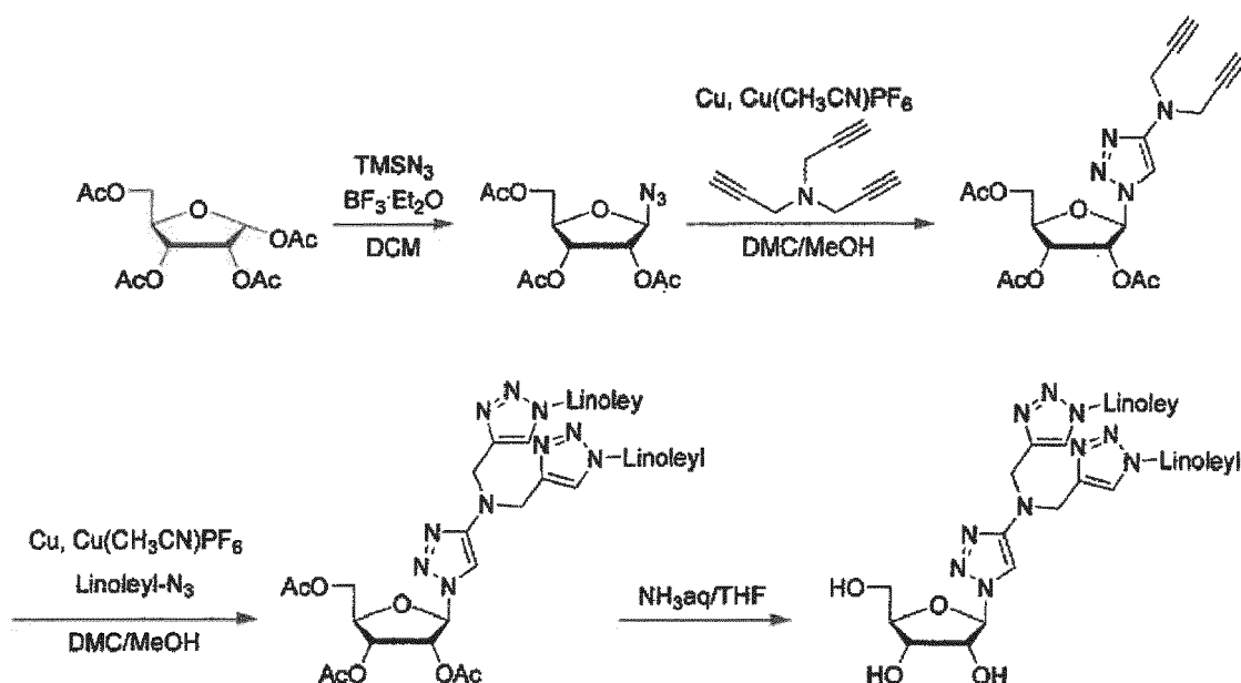
Scheme 38
