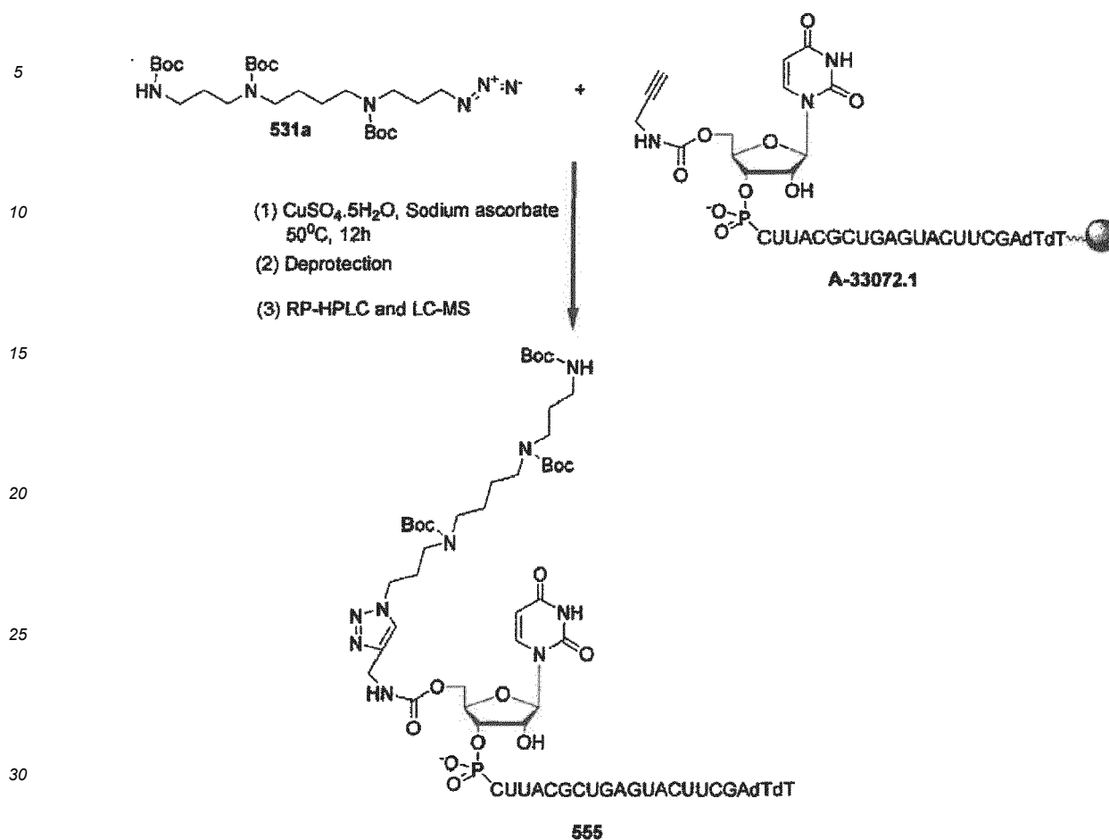
Scheme 44
