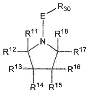
Formula (VI)
