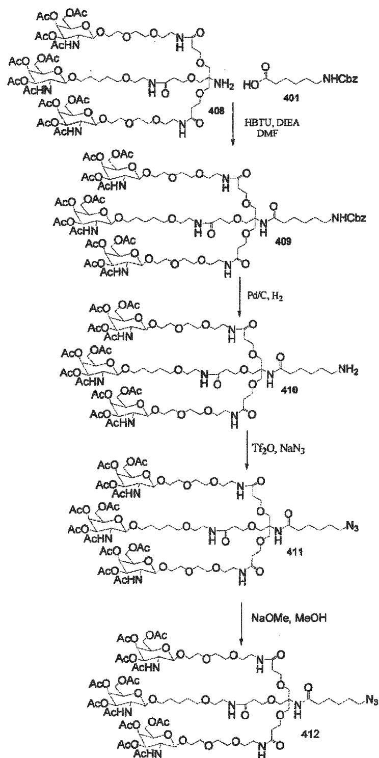
Scheme 18
