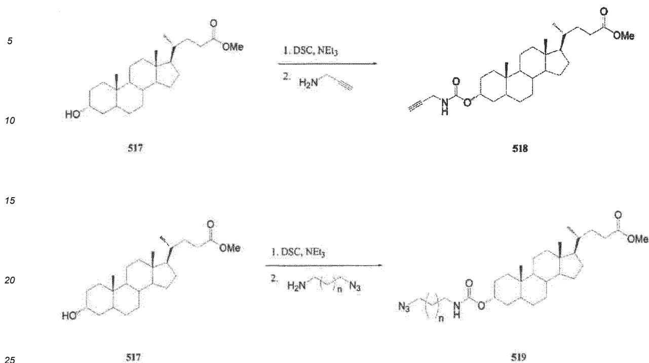
Scheme 32
