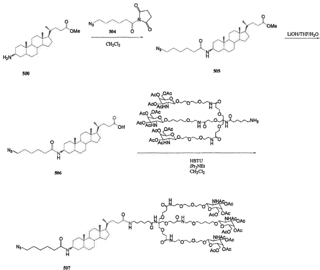
Scheme 29
