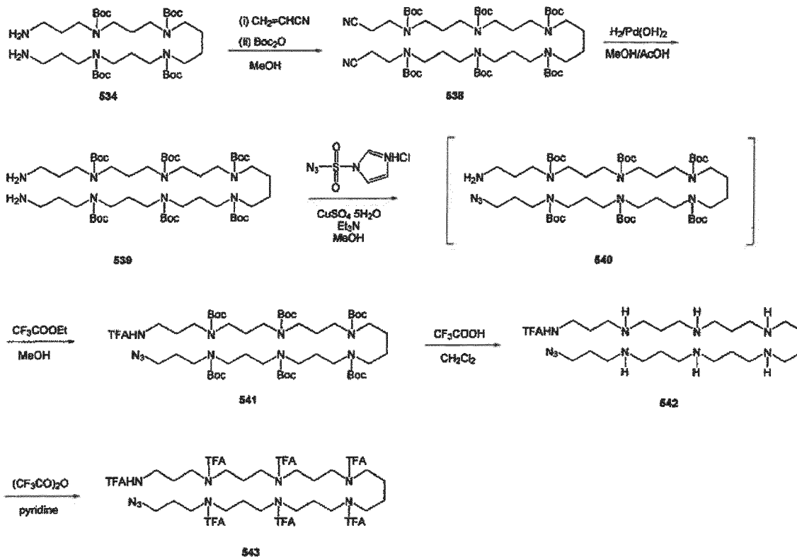
Scheme 37
