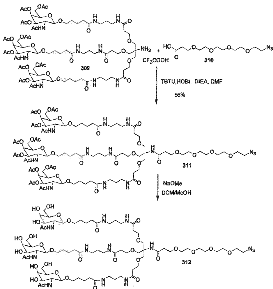
Scheme 11
