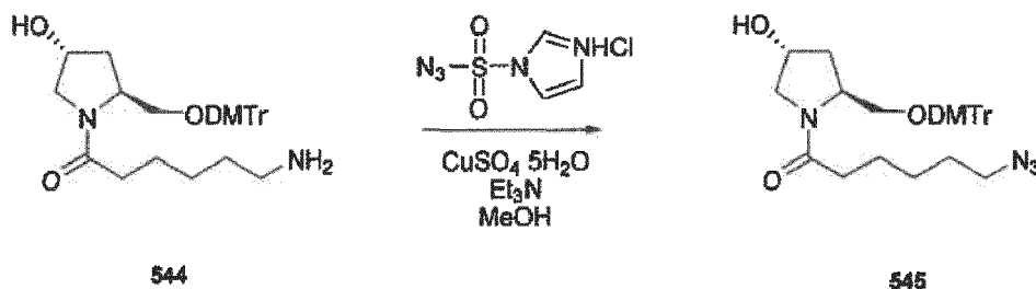
Scheme 41
