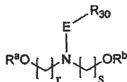
Formula (VIII)
