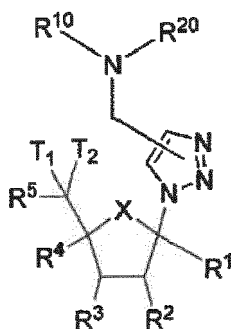
Formula (IVa)
