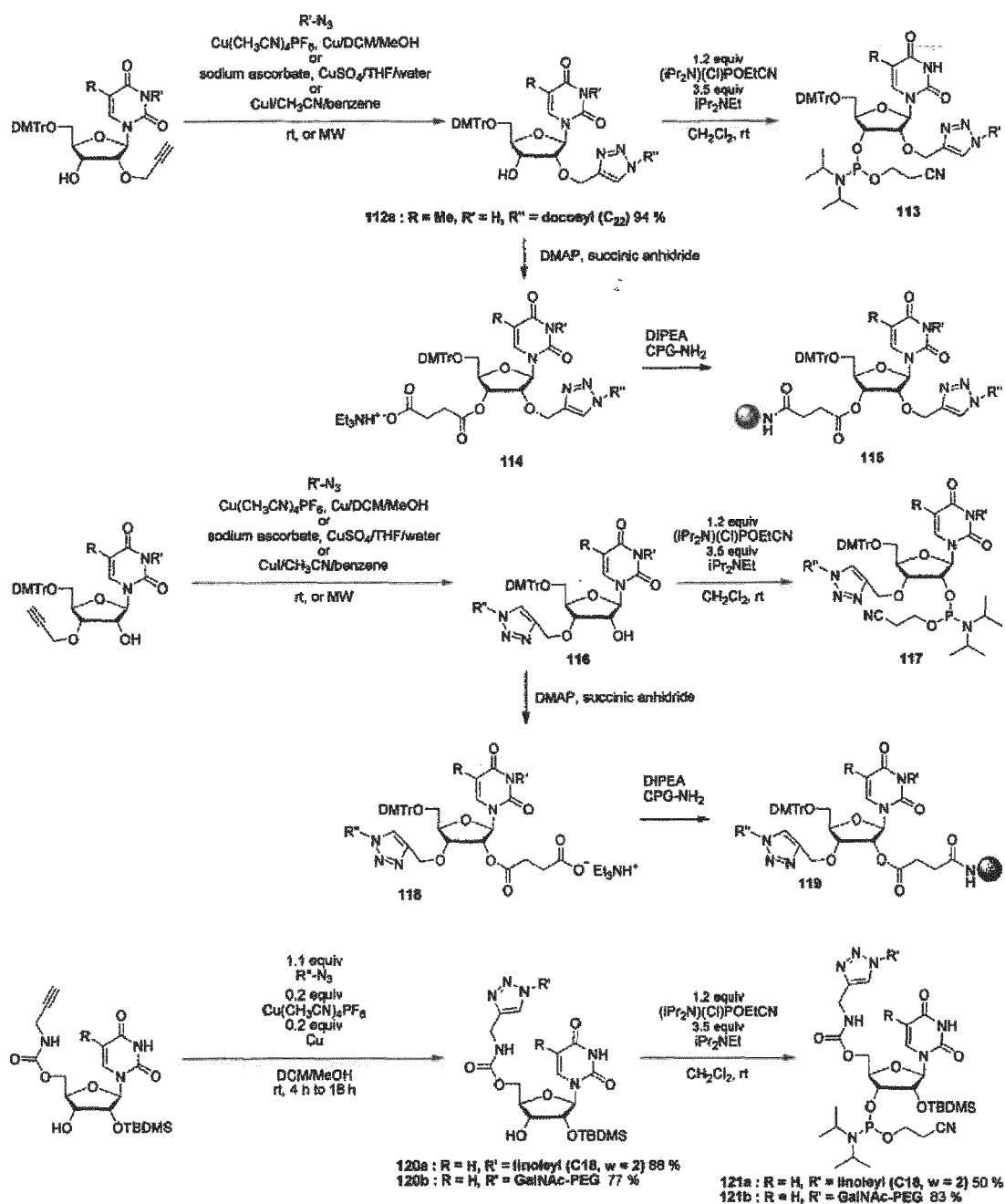
Scheme 9
