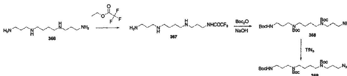
Scheme 27
