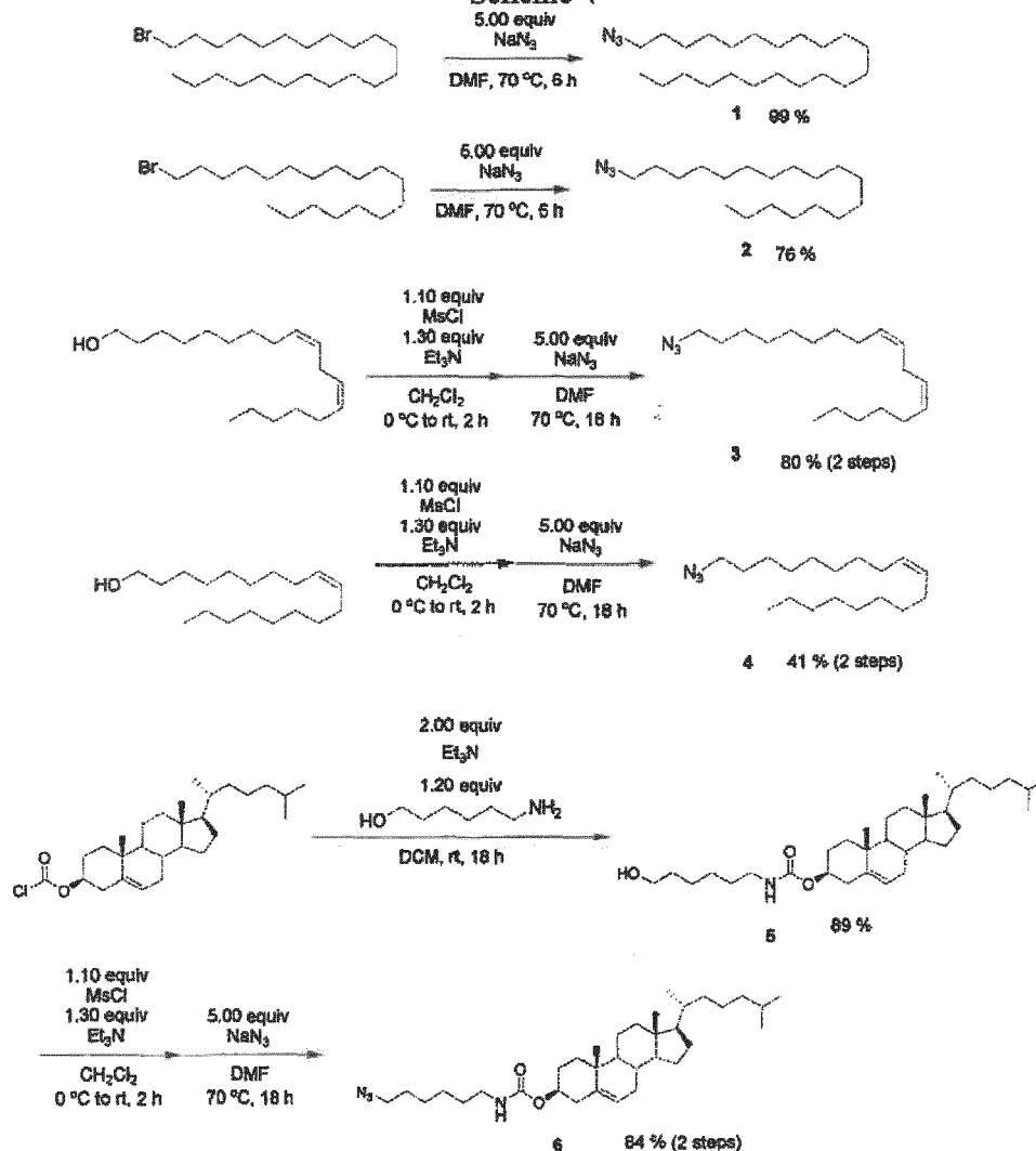
Scheme 4
