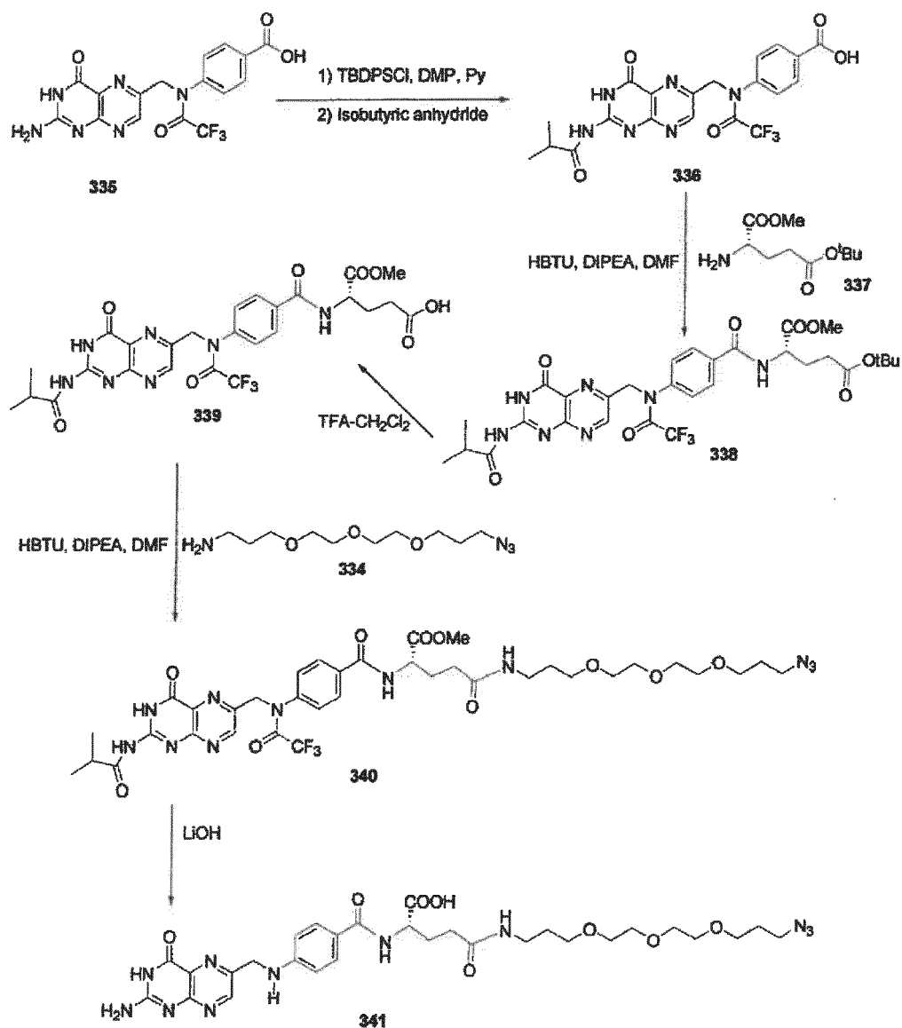
Scheme 21
