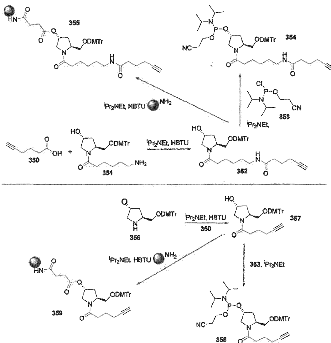
Scheme 25
