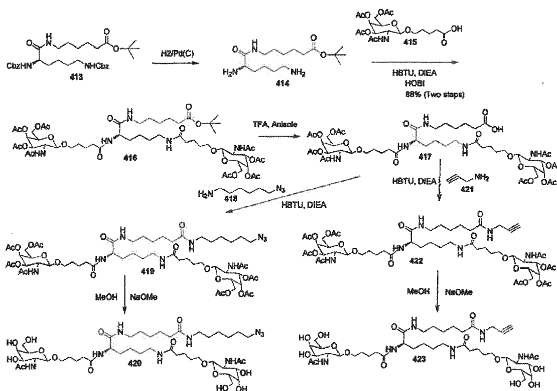
Scheme 19
