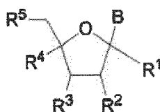
Formula (III)
