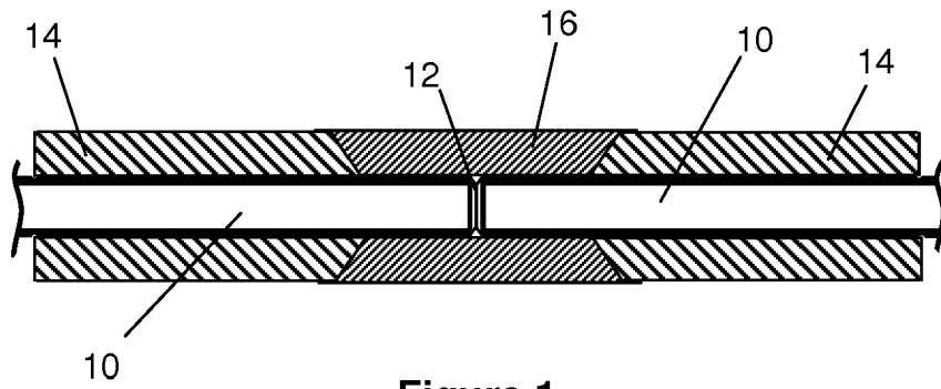
Figure 1 PRIOR ART
