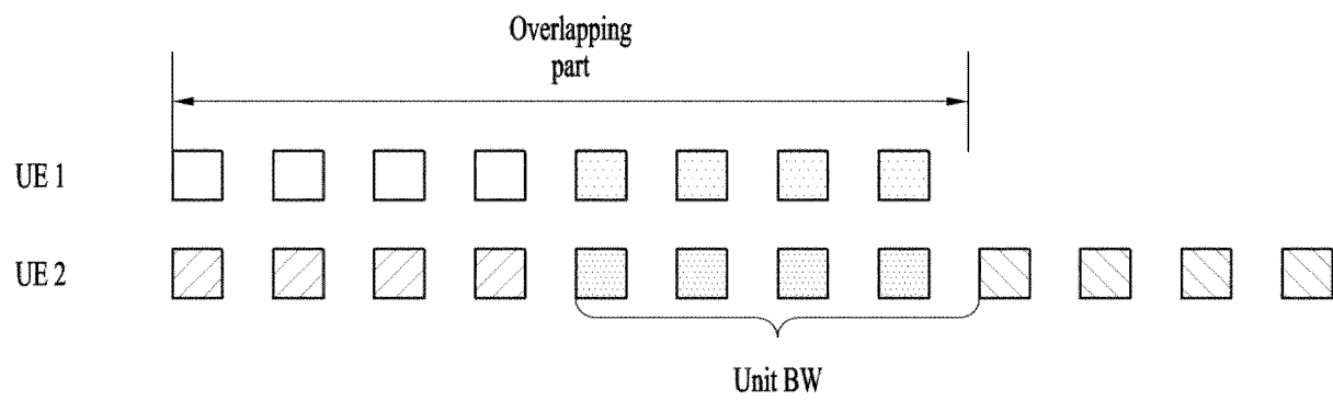
(b) An example of overlapping two SRS units
