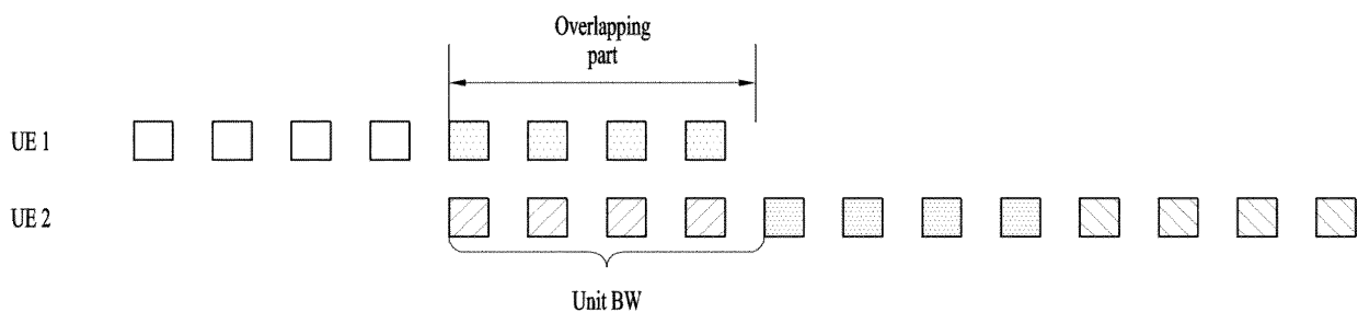
(a) An example of overlapping one SRS unit
