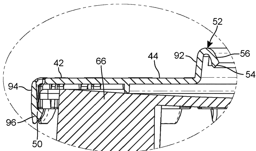
DETAIL B SCALE 2 : 1 FIG. 15C
