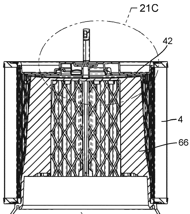
SECTION C1-C1
