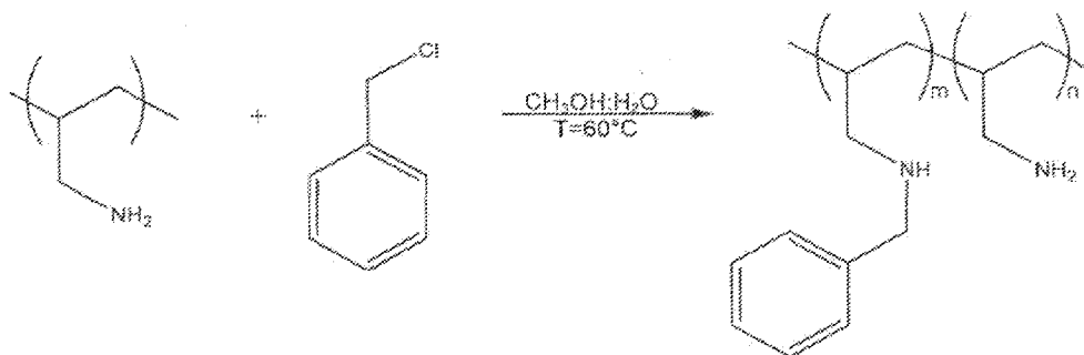
Figure 1. Reaction of polyallylamine with benzylchloride. The letters "m" and "n" represent the different types of monomer units in the polyelectrolyte backbone.
