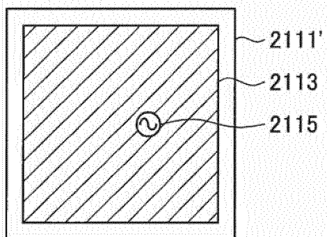
PATCH ANTENNA
