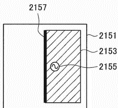
SHORT-CIRCUIT PATCH ANTENNA
