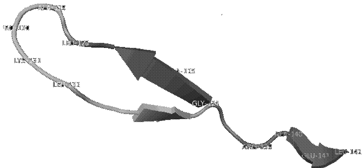
Figure 2C. PD-1:92-110: ^{92}\text{G-A-I-S-L-A-P-K-A-Q-I-K-E-S-L-R-A-E-L}^{110}
