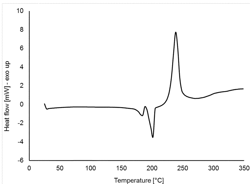
Figure 3: DSC scan
