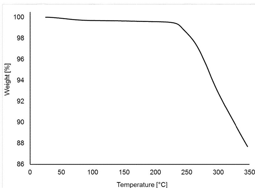
Figure 4: TGA profile
