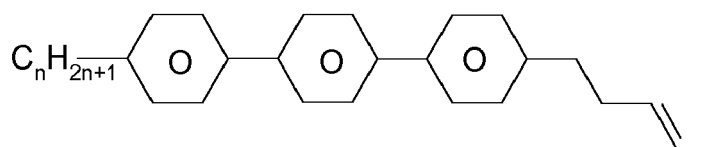
PPP-n-2V1
