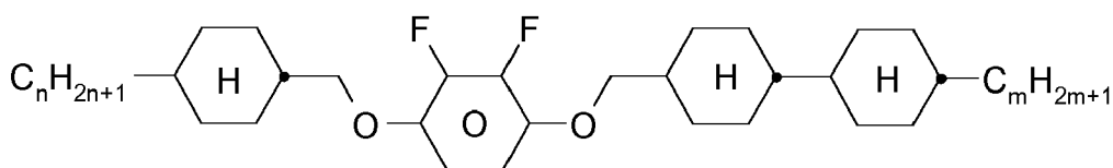
COYOICC-n-m
