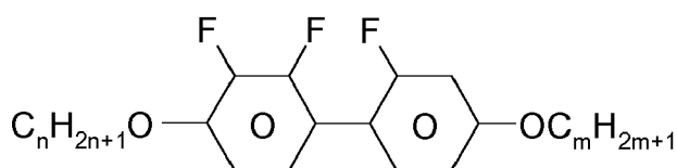
YGI-nO-Om
