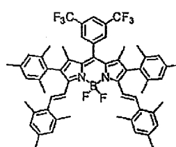
Compound (3)
