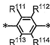
Formula (L - 3)
