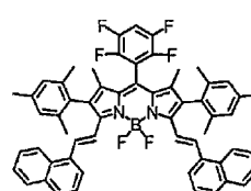
Compound (11)
