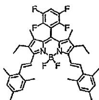
Compound (6)
