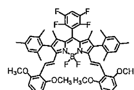
Compound (12)
