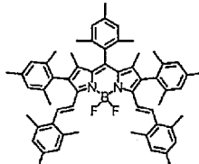
Compound (10)
