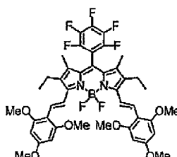
Compound (7)
