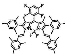
Compound (5)
