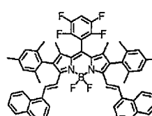
Compound (11)
