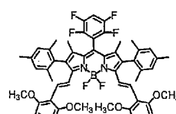
Compound (12)
