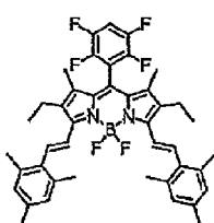
Compound (6)
