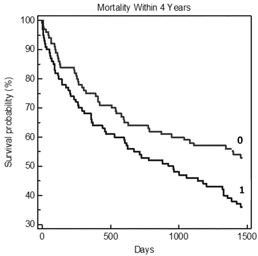
Figure 1B: Galectin-3 K-M Analysis for 4 Years (log rank p=0.020 )
