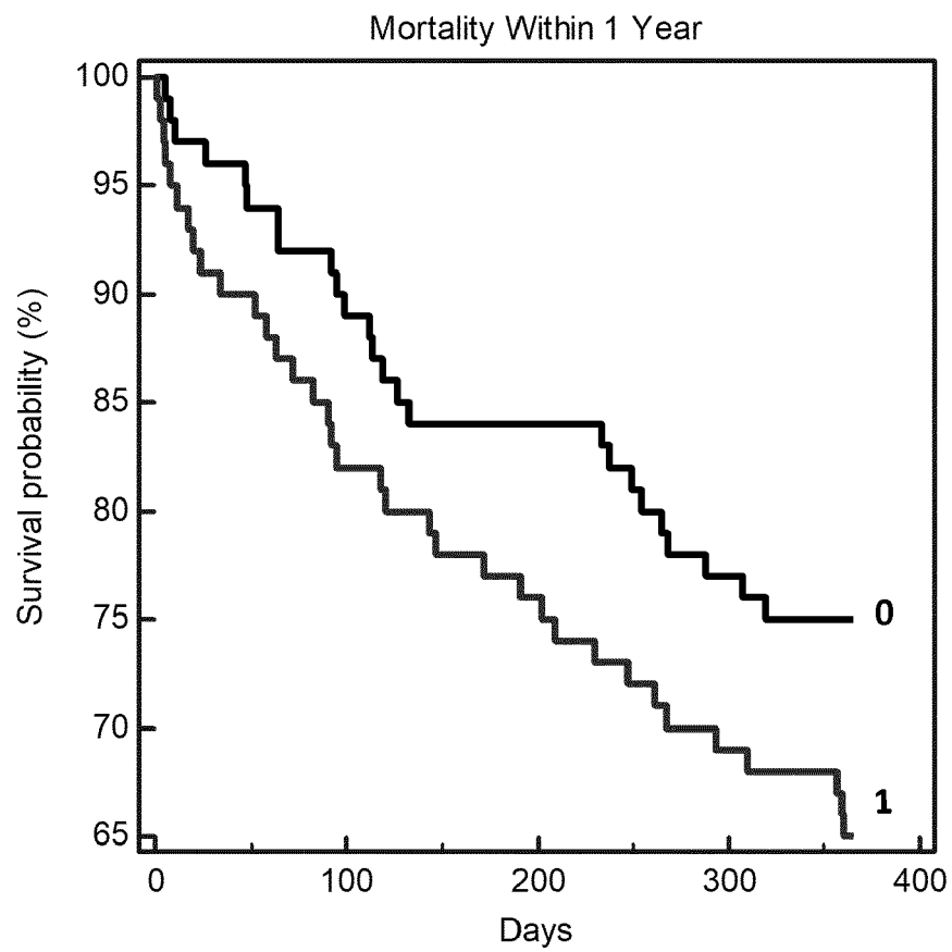
Figure 1A: Galectin-3 K-M Analysis for 1 Year (log rank p=0.1122)
