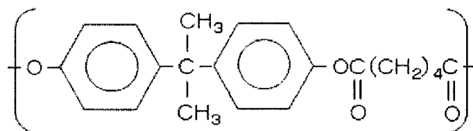
Structural Formula (G)
