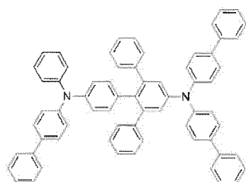
[Chemical Formula 30]
