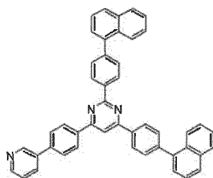
[Chemical Formula 40]
