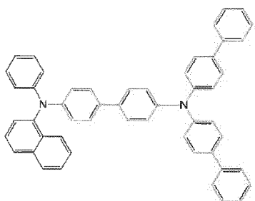
[Chemical Formula 7]
