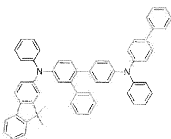
[Chemical Formula 27]
