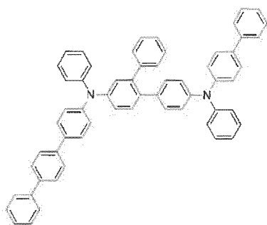
[Chemical Formula 31]
