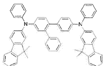
[Chemical Formula 21]
