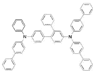
[Chemical Formula 16]
