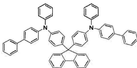
[Chemical Formula 44]
