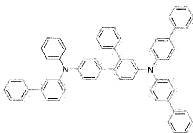
[Chemical Formula 25]
