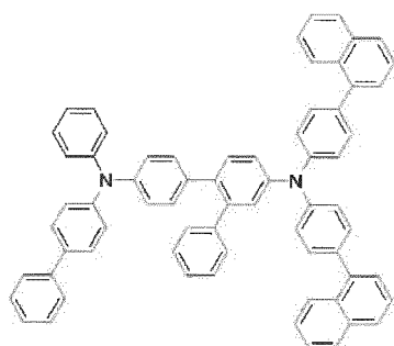
[Chemical Formula 19]
