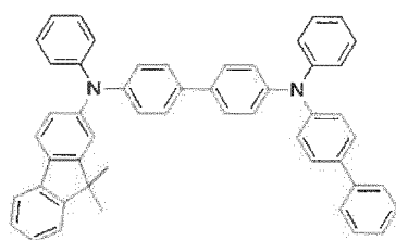
[Chemical Formula 24]
