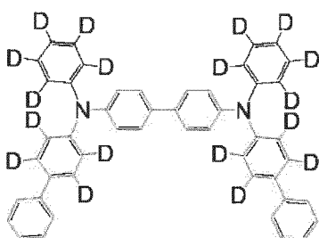
[Chemical Formula 11]
