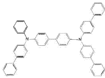
[Chemical Formula 4]
