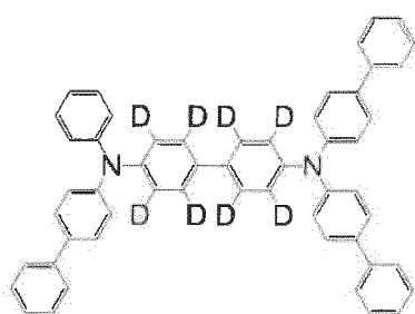
[Chemical Formula 15]
