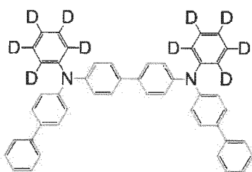
[Chemical Formula 9]
