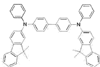
[Chemical Formula 23]
