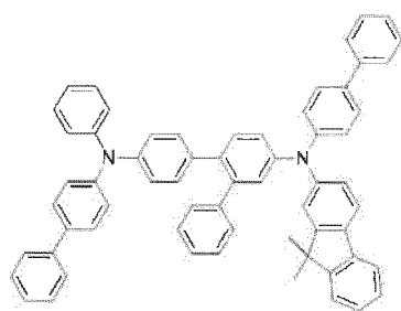
[Chemical Formula 20]
