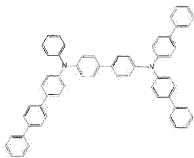
[Chemical Formula 6]
