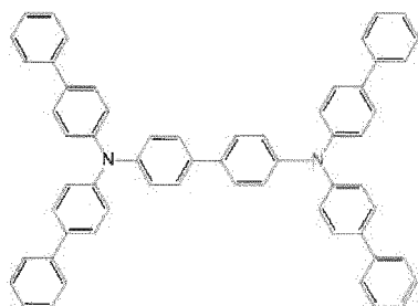
[Chemical Formula 45]
