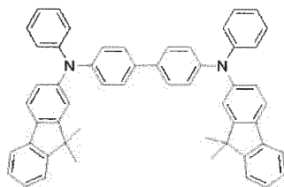
[Chemical Formula 35]
