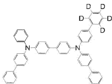
[Chemical Formula 13]
