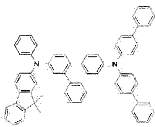
[Chemical Formula 28]
