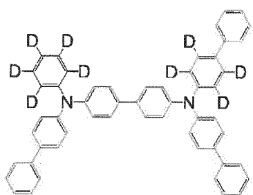
[Chemical Formula 12]
