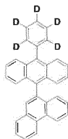
[Chemical Formula 39]
