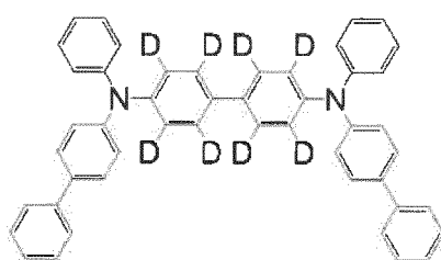
[Chemical Formula 10]
