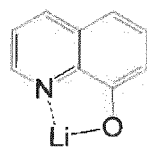
[Chemical Formula 41]
