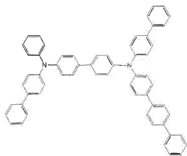
[Chemical Formula 5]
