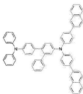
[Chemical Formula 32]
