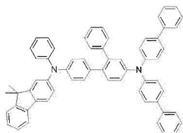
[Chemical Formula 29]
