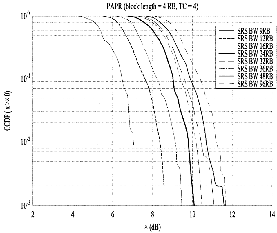
SRS BW dependent PAPR (block length=4RB, TC=4)
