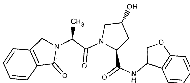
Isomer 1
