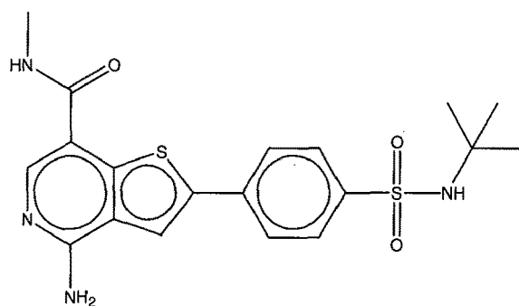
6TP
