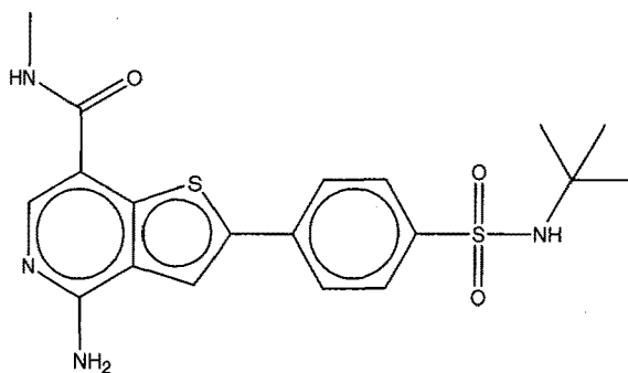
6TP
