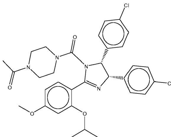
Nutlin-1
