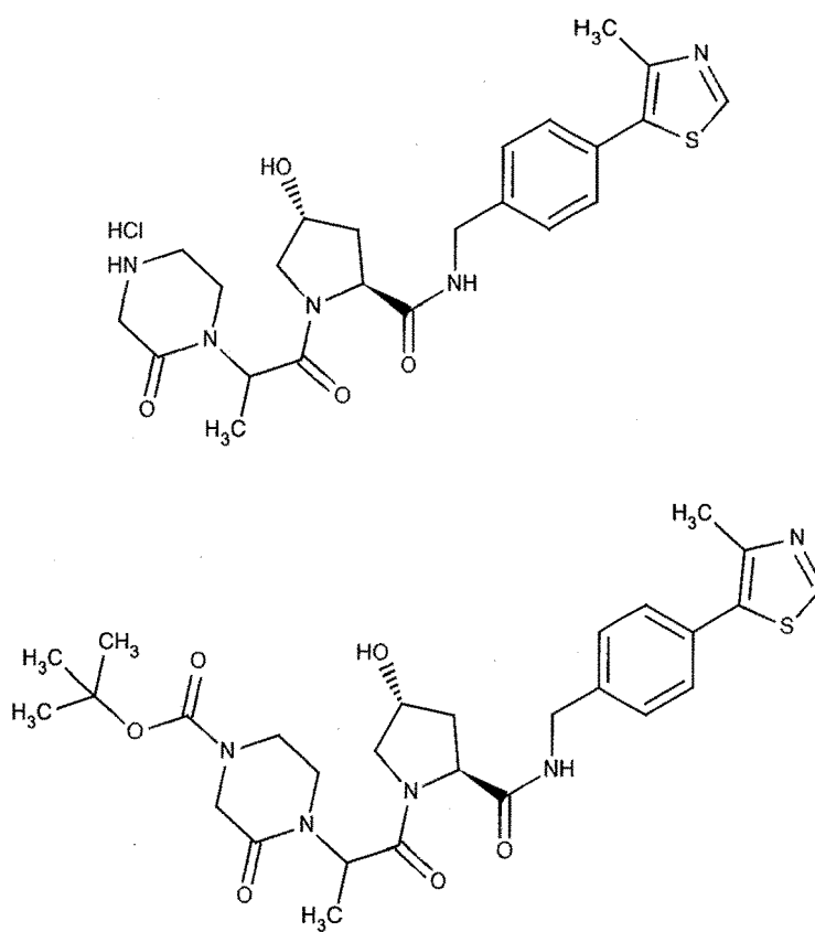
Isomer 2
