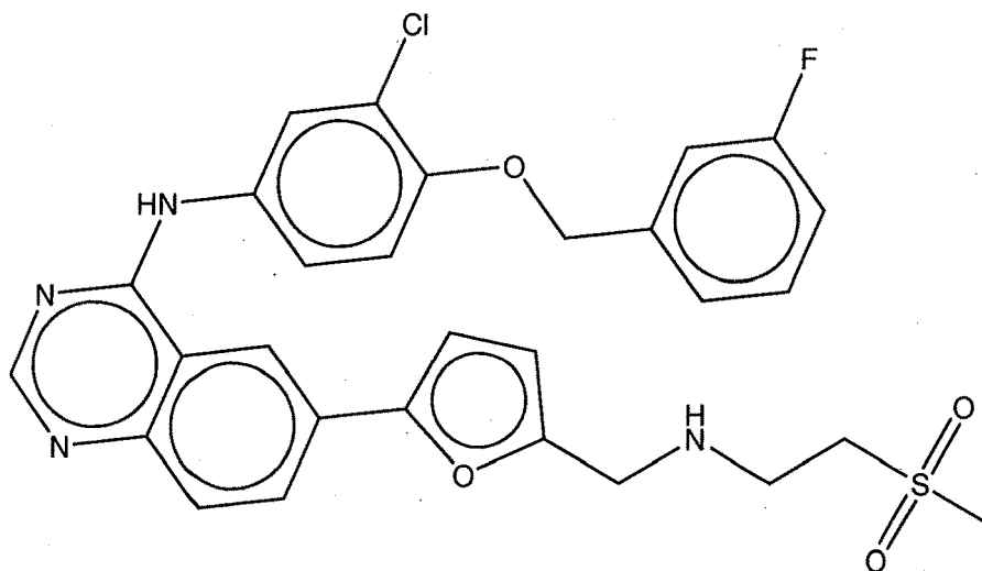
Lapatinib
