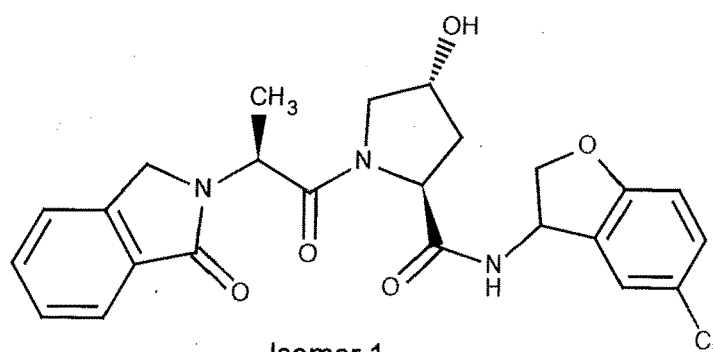
Isomer 1
