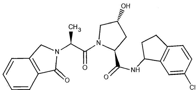
Isomer 2
