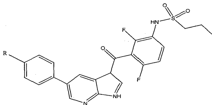
PLX4032,
