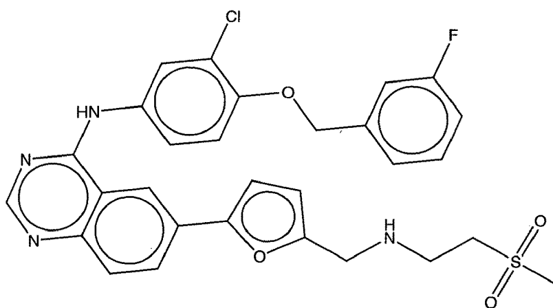
Lapatinib
