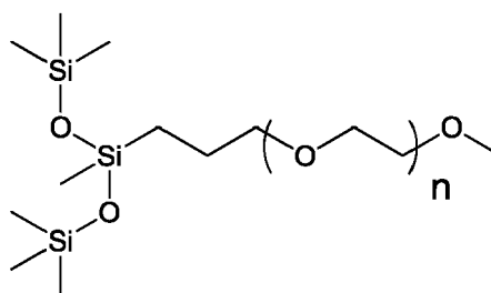
(Compound I: polyalkyleneoxide heptamethyltrisiloxane, average n=7.5 ).
