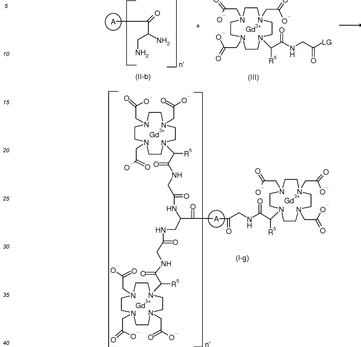
Scheme 7: Route for the preparation of compounds of general formula (I-g), wherein
