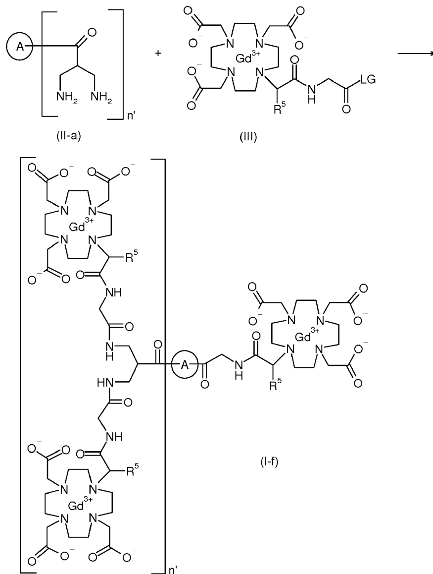
Scheme 6: Route for the preparation of compounds of general formula (I-f), wherein
