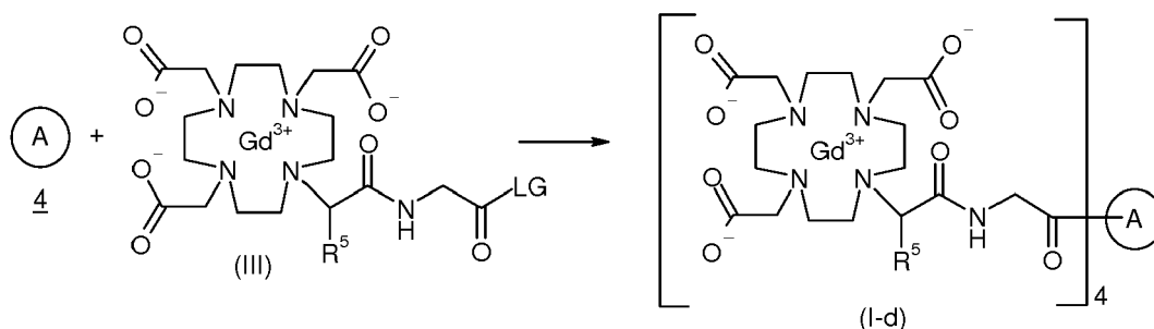
Scheme 4: Route for the preparation of compounds of general formula (I-d), wherein R^5 has the meaning as given for general formula (I), supra ,
