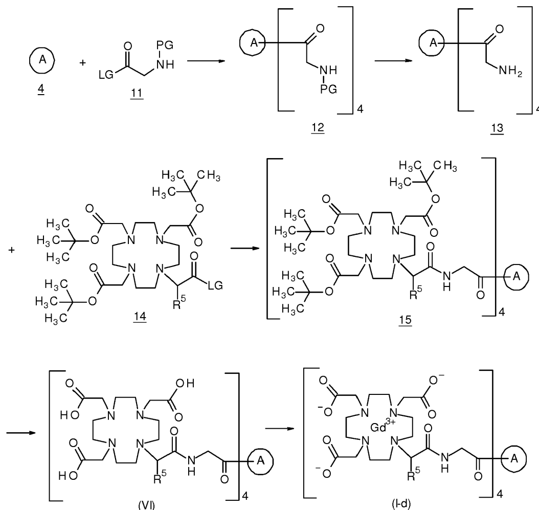
Scheme 11: Alternative route for the preparation of compounds of general formula (I-d), wherein R^5 has the meaning as given for general formula (I), supra ,
