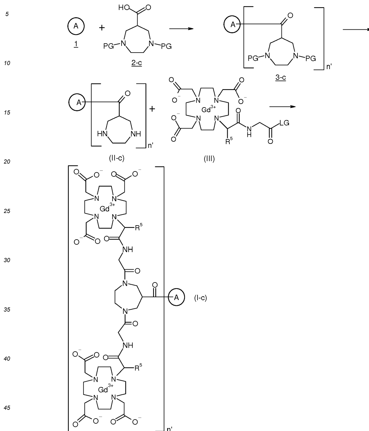
Scheme 3: Route for the preparation of compounds of general formula (I-c), wherein
