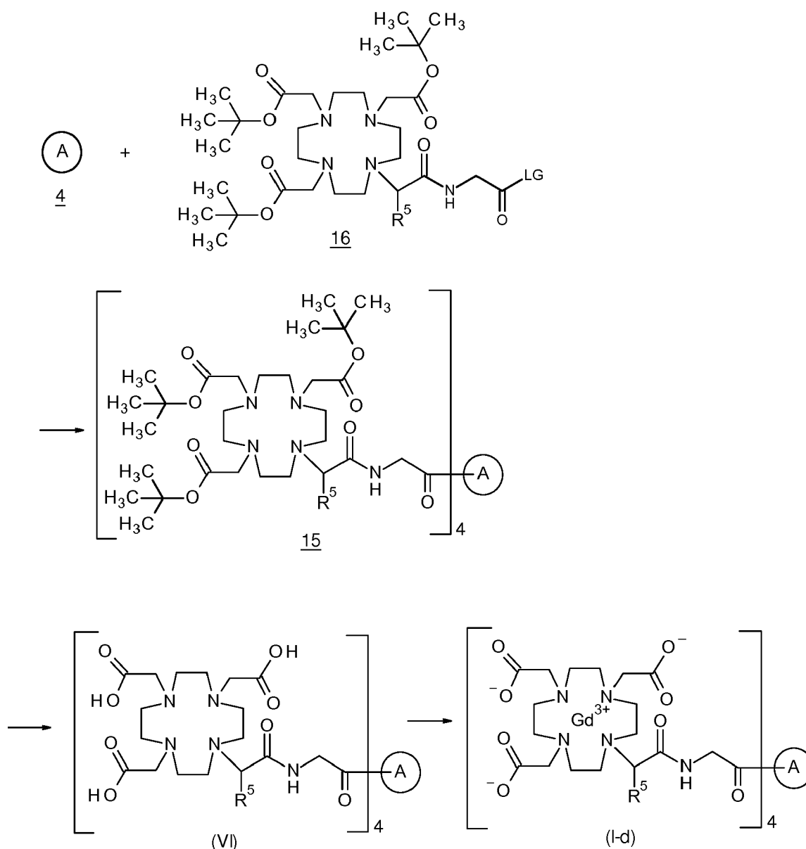
Scheme 12: Alternative route for the preparation of compounds of general formula (I-d), wherein R^5 has the meaning as given for general formula (I), supra ,
