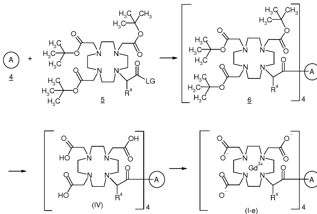
Scheme 5: Route for the preparation of compounds of general formula (I-e), wherein R^4 has the meaning as given for general formula (I), supra ,
