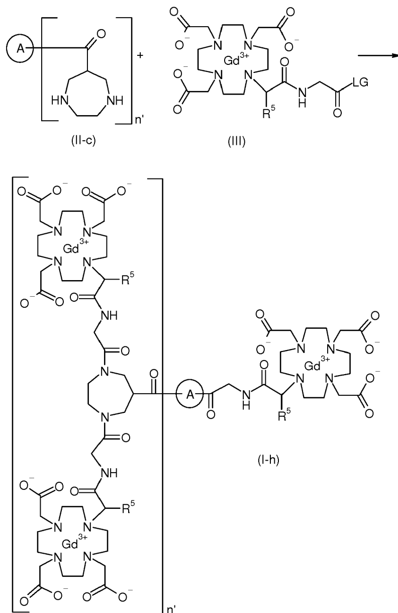
Scheme 8: Route for the preparation of compounds of general formula (I-h), wherein
