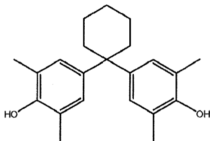
1,1-di(4-hydroxy-3,5-dimethylphenyl)-cyclohexane.
