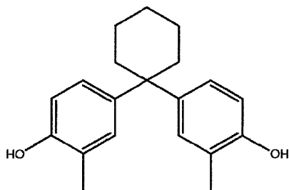
1,1-di(4-hydroxy-3-methylphenyl)-cyclohexane
