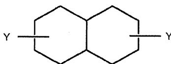
bicyclo[4.4.0]decane
