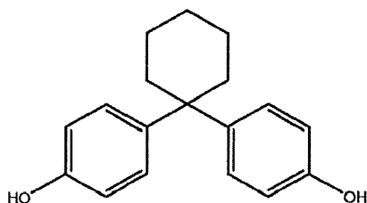
1,1-di(4-hydroxyphenyl)-cyclohexane
