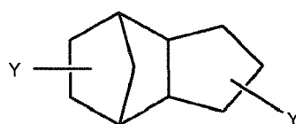
tricyclodecane
