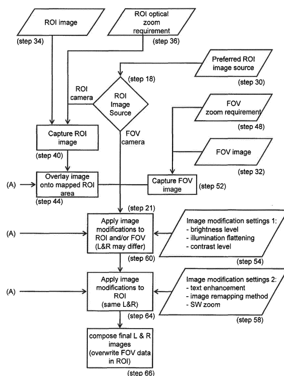
Figure 6-2 Process Steps (per frame)
