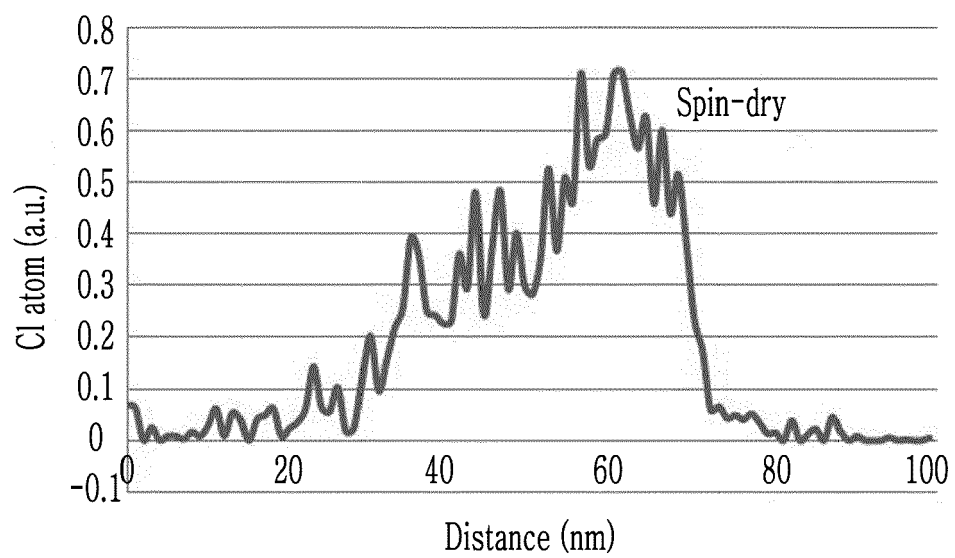
Cl distribution
