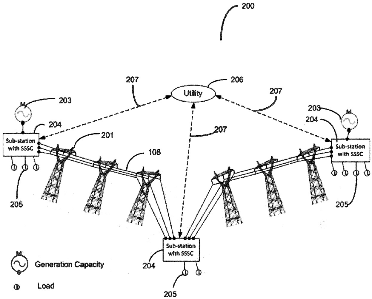
Fig. 2 (PRIOR ART)
