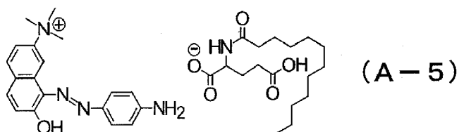
[Chem. 10]
