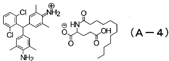
[Chem. 10]
