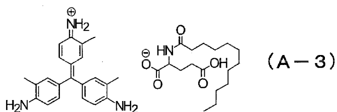
[Chem. 8]
