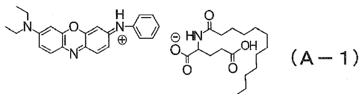
[Chem. 7]
