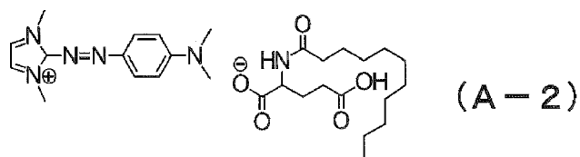
[Chem. 8]
