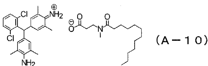
[Chem. 16]
