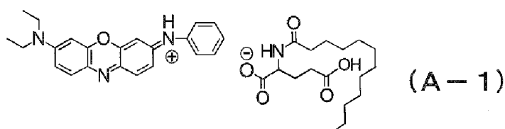
[Chem. 7]
