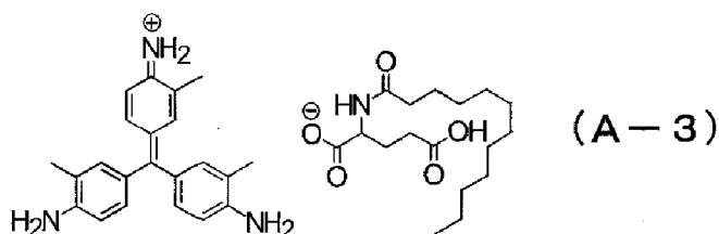
[Chem. 8]
