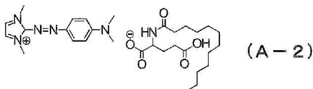
[Chem. 8]
