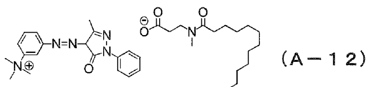
[Chem. 17]
