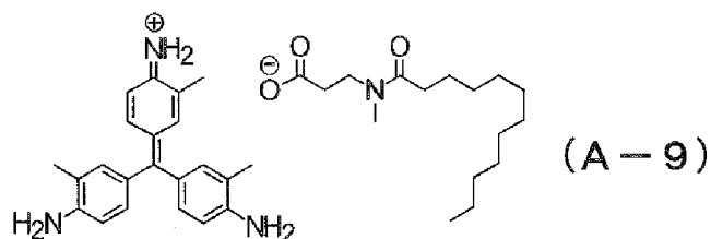
[Chem. 14]
