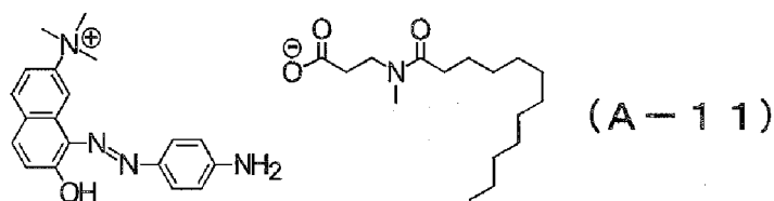
[Chem. 17]
