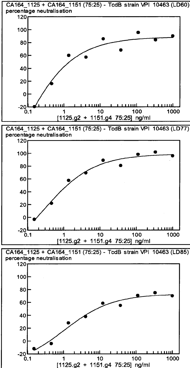
Figure 44 Anti TcdB (Ribotype 003) in-vitro neutralization data for two Mab mixtures at different relative Mab ratios and different toxin concentrations
