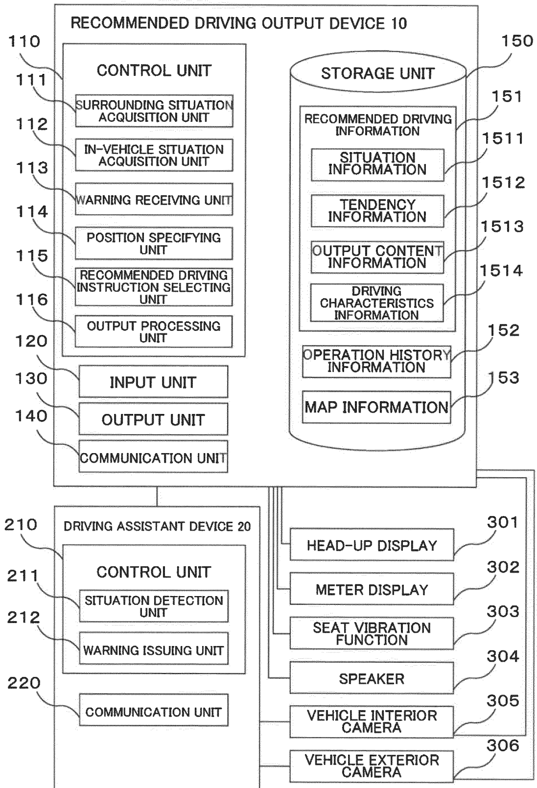
FIG. 2 RECOMMENDED DRIVING OUTPUT SYSTEM 1
