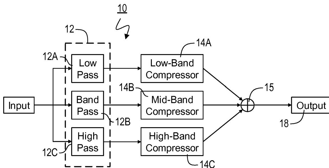
FIG. 1 (Prior Art)
