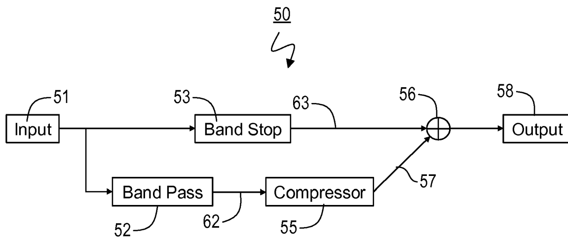
FIG. 4 (Prior Art)
