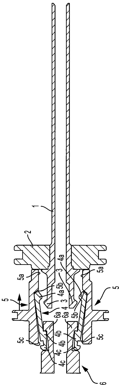
Fig. 2 Prior Art
