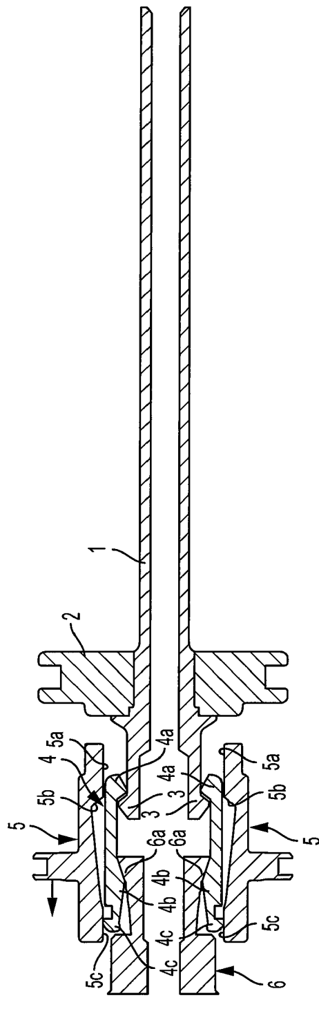
Fig. 1 Prior Art
