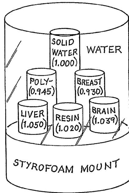
ELECTRON DENSITY PHANTOM (CONTRAST, CT LINEARITY)
