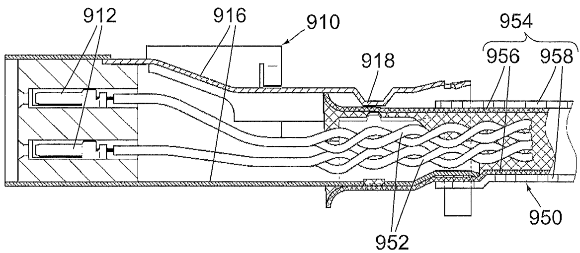
FIG.15 PRIOR ART
