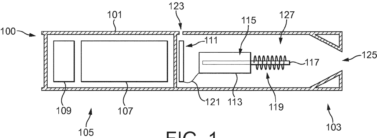
FIG. 1 (PRIOR ART)
