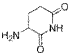
[Chemical formula 3]
