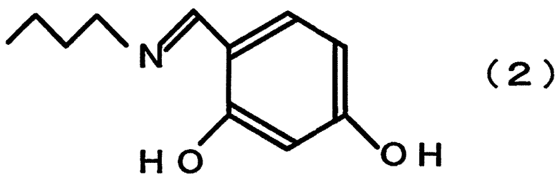
[Chem. 2]
