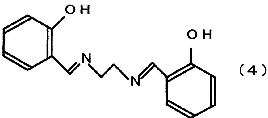
[Chem. 4]
