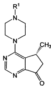
Formula I,
