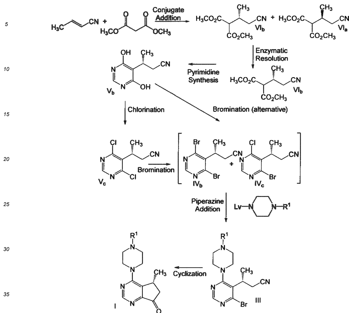
Scheme 3
