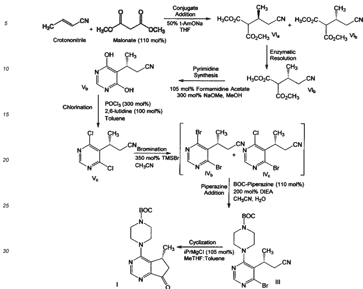
Scheme 4
