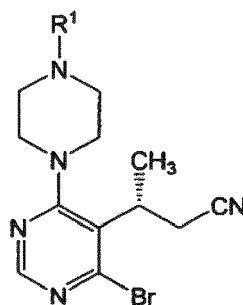
Formula III,
