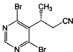
Formula IV b ,
