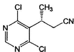
Formula V c ,
