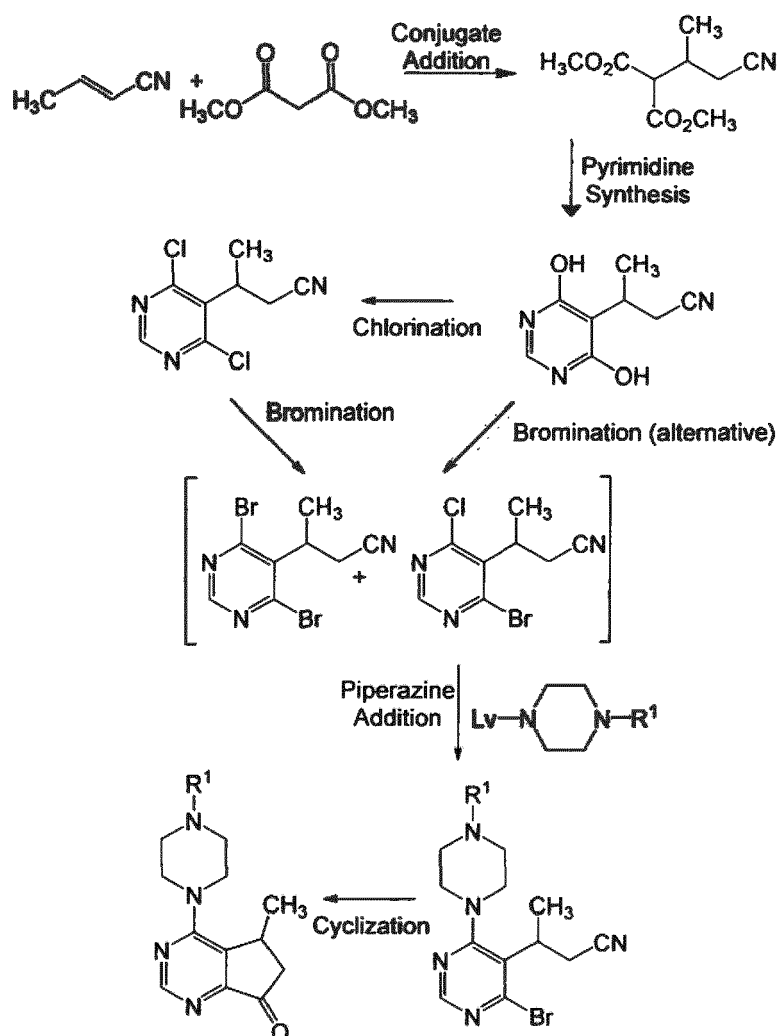
Scheme 2
