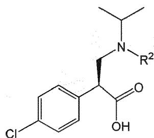
Formula VIII,
