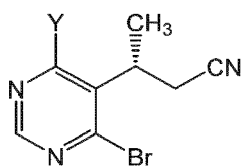
Formula IV,
