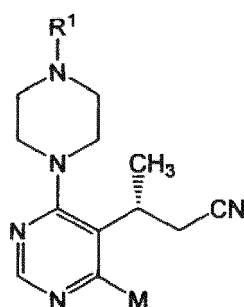
Formula II,
