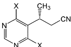
Formula V,
