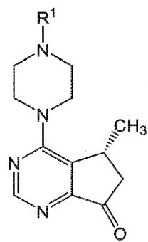
Formula I,
