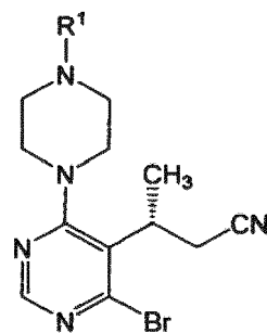
Formula III,
