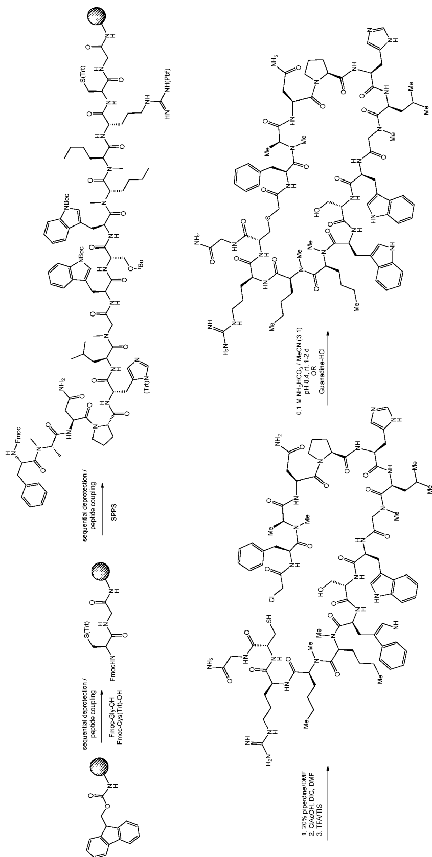
SCHEME 1 - COMMON SYNTHETIC METHOD USED FOR THIOETHER-CYCLIZED PEPTIDES (EXAMPLES 2 THRU 88)
