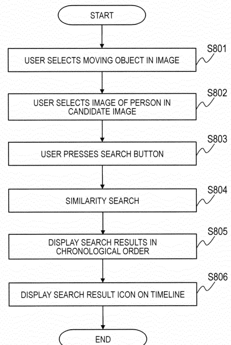
MOVING OBJECT SEARCH PROCESS FLOWCHART
