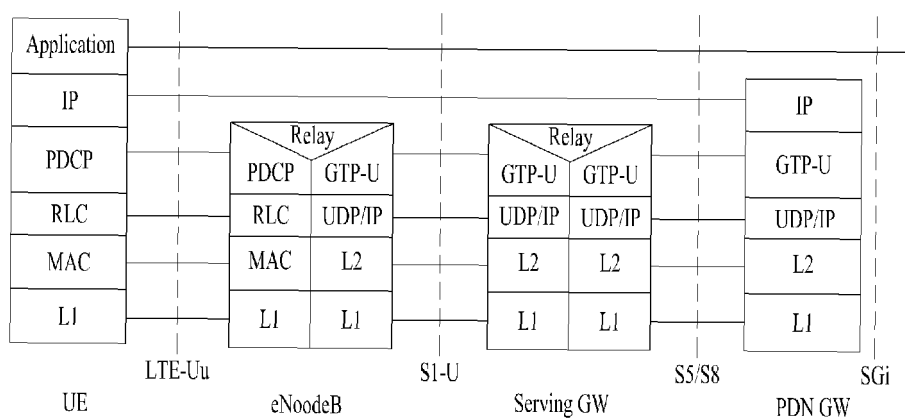
(a) UE-P-GW user plane with E-UTRAN
