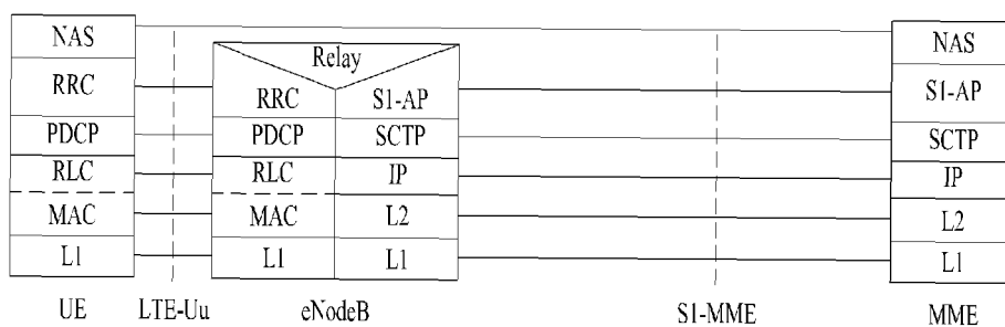
(b) Control Plane UE-MME
