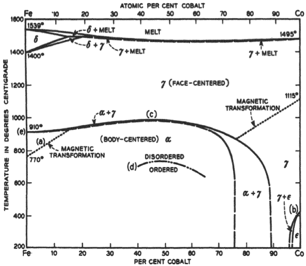
Phase diagram of iron-cobalt alloys.
