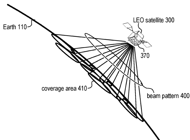
FIG. 4 Multiple-beam pattern 400 from LEO satellite 300
