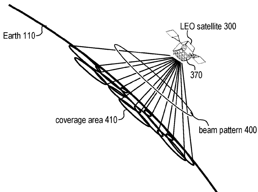
FIG. 4 Multiple-beam pattern 400 from LEO satellite 300
