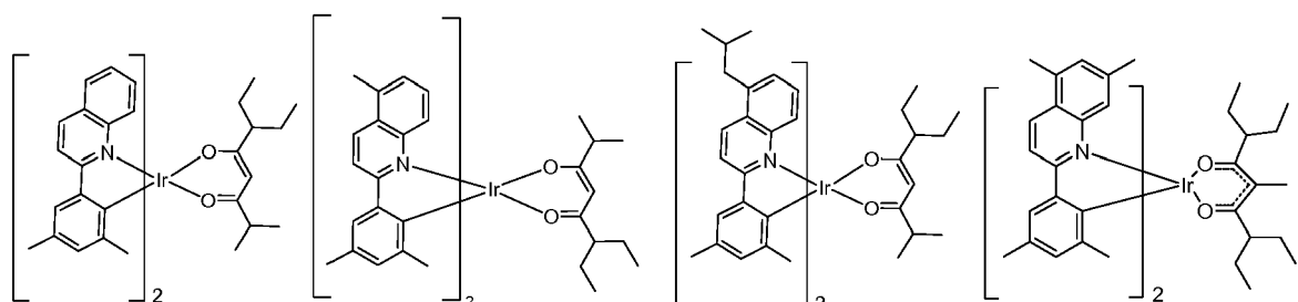
Compound 141 , Compound 142 , Compound 176 , Compound 278 ,
