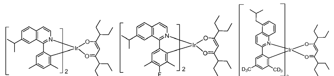
Compound 83 , Compound 93 , Compound 118 ,
