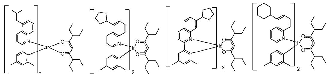
Compound 43 , Compound 54 , Compound 55 , Compound 62 ,
