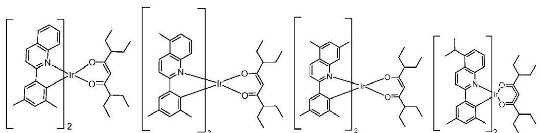
Compound 8 , Compound 9 , Compound 12 , Compound 32 ,
