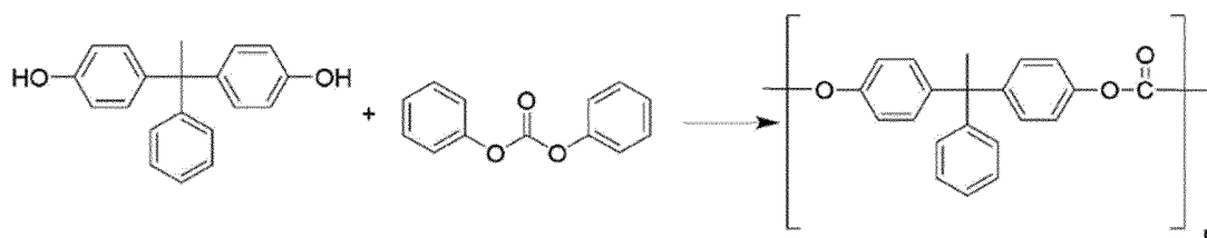
[Chemical Formula 6]
