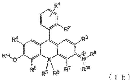
[Chemical Formula 23]
