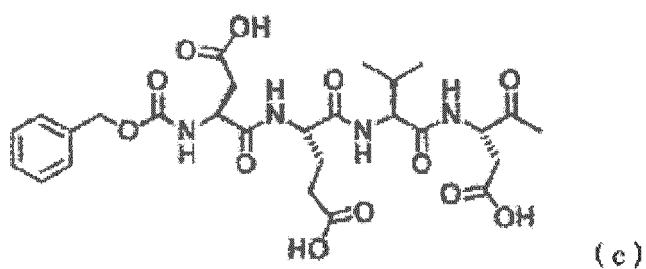
[Chemical Formula 26]
