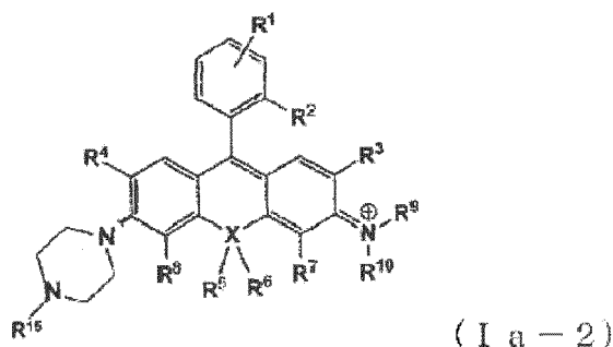
[Chemical Formula 22]
