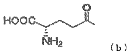
[Chemical Formula 25]
