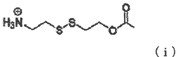
[Chemical Formula 29]
