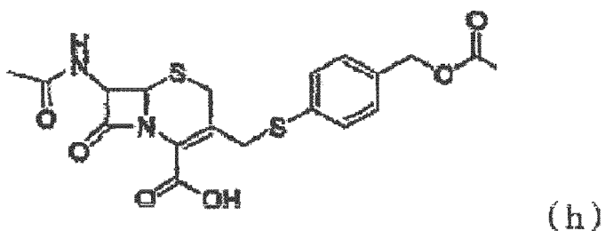
[Chemical Formula 28]
