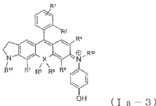
[Chemical Formula 31]
