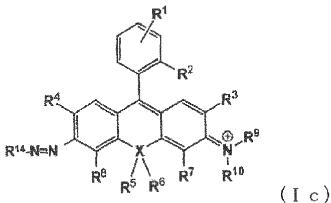
[Chemical Formula 30]
