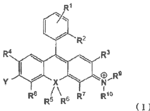
[Chemical Formula 1]
