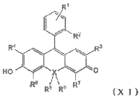
[Chemical Formula 15]
