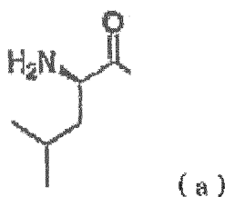
[Chemical Formula 24]
