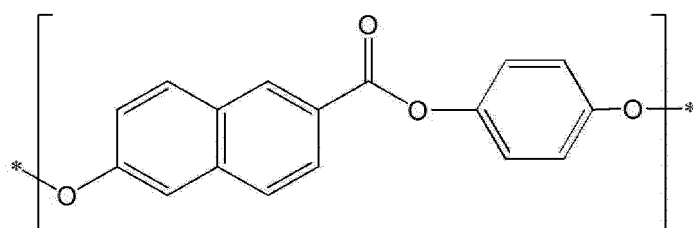
[Chemical Formula 10-1]
