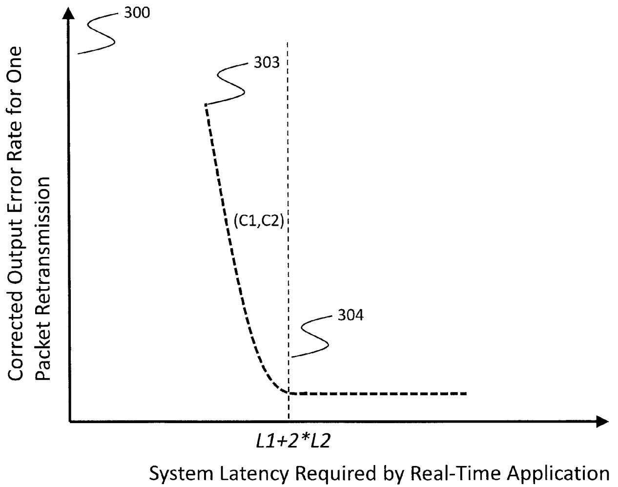
Figure 3. Combined Latency versus Output Error Rate
