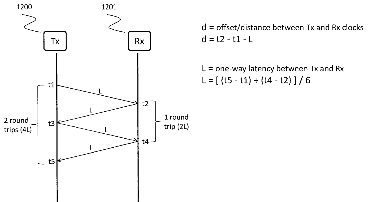
Figure 12. Transmitter/Receiver Clock synchronization Diagram
