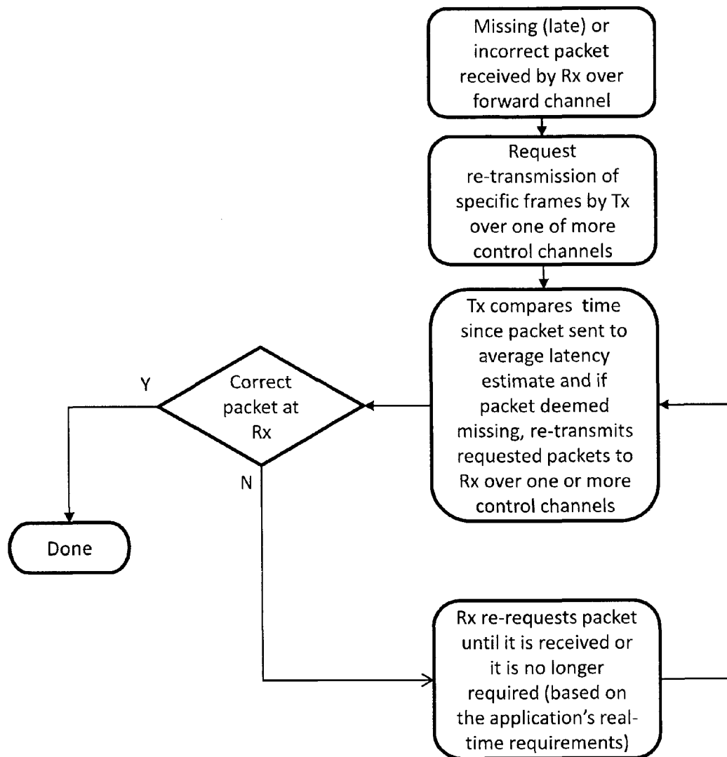
Figure 4. Error Correction via Packet Re-transmission
