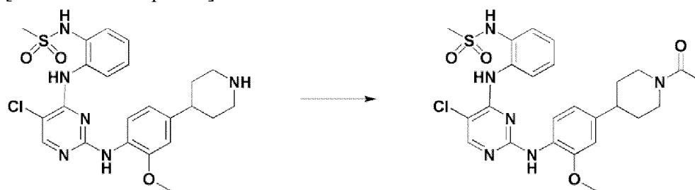
[Reaction Example 14]
