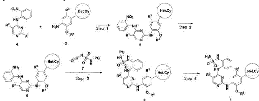
[Reaction Scheme 2]
