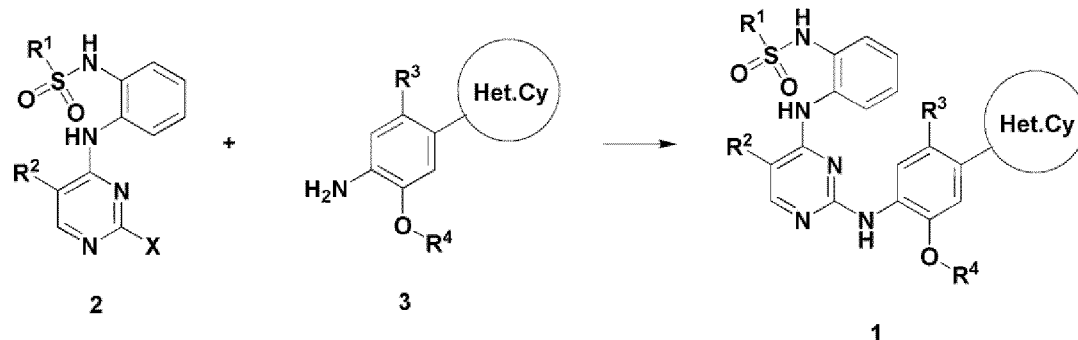
[Reaction Scheme 1]
