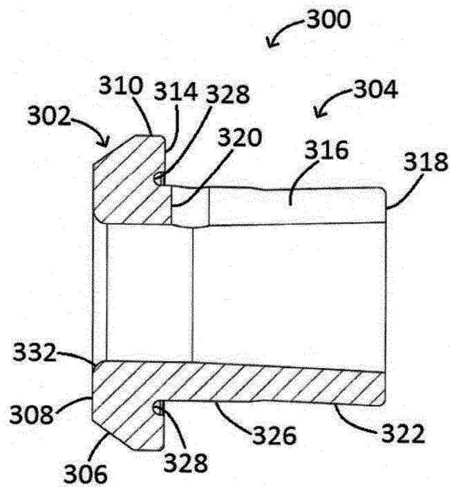
SECTION B-B
