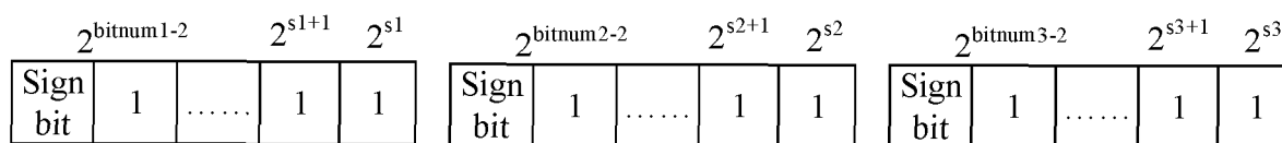
Fixed-point data 1
